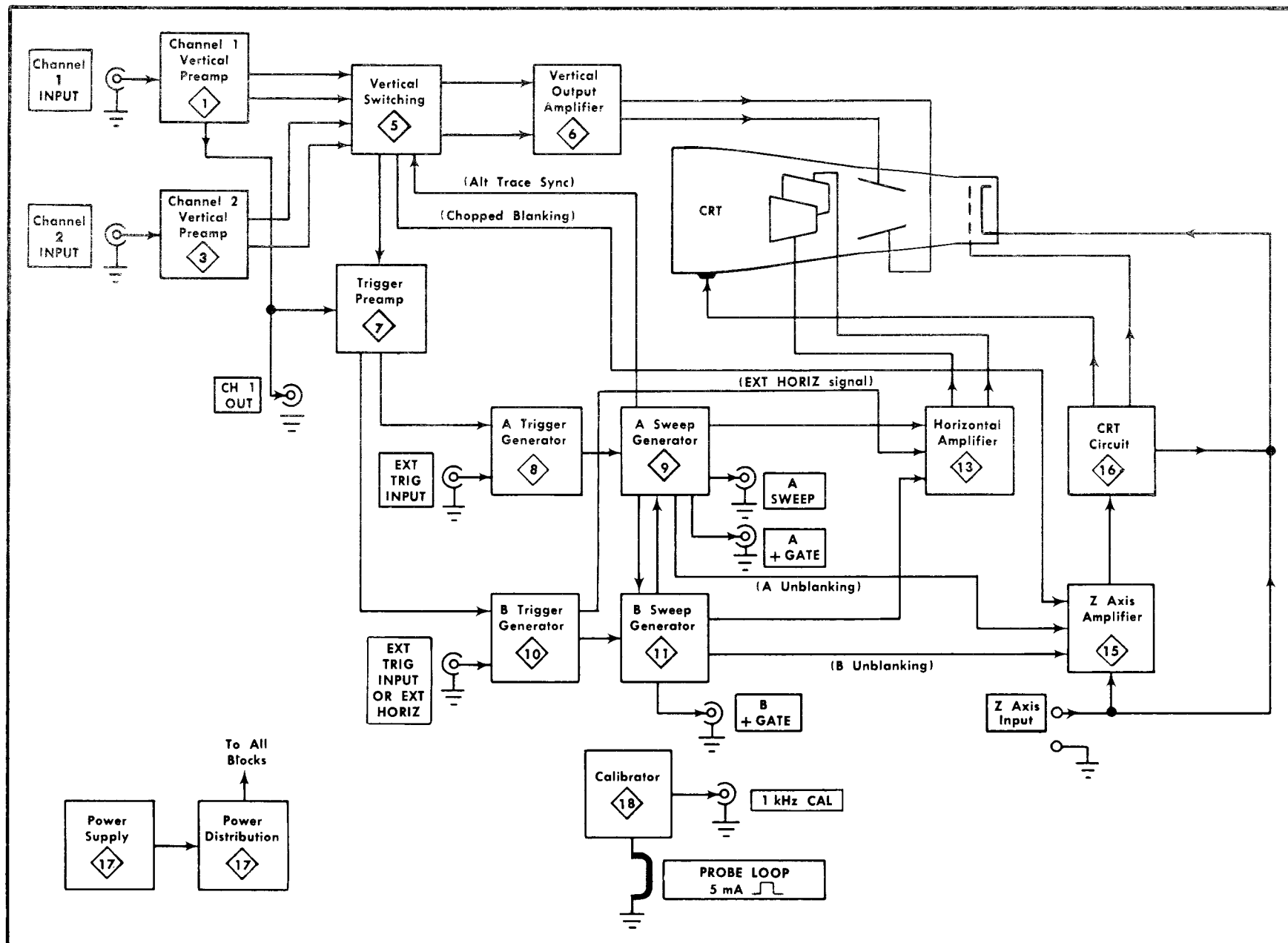
Fig. 3-1. Basic block diagram of the Type 453.
