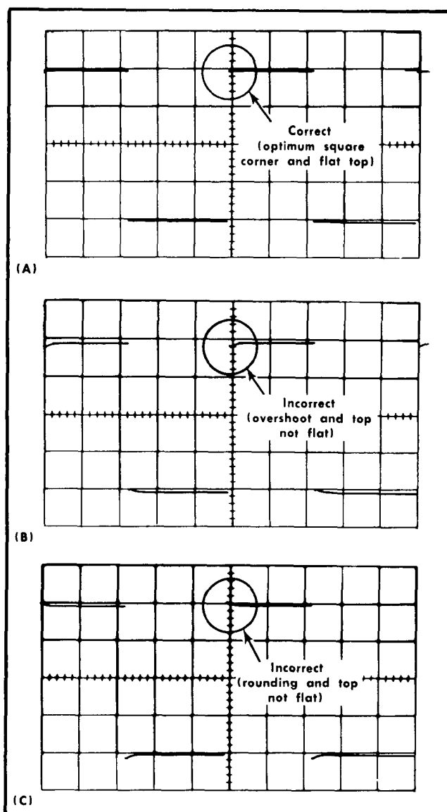
Fig. 5-5. (A) Typical CRT display showing correct compensation, (B) and (C) incorrect compensation.
