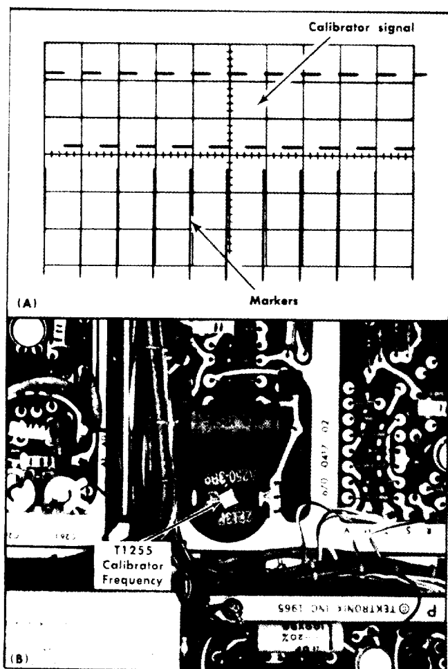
Fig. 6-56. (A) Typical CRT display showing correct calibrator repetition rate, (B) location of Calibrator Frequency adjustment.
