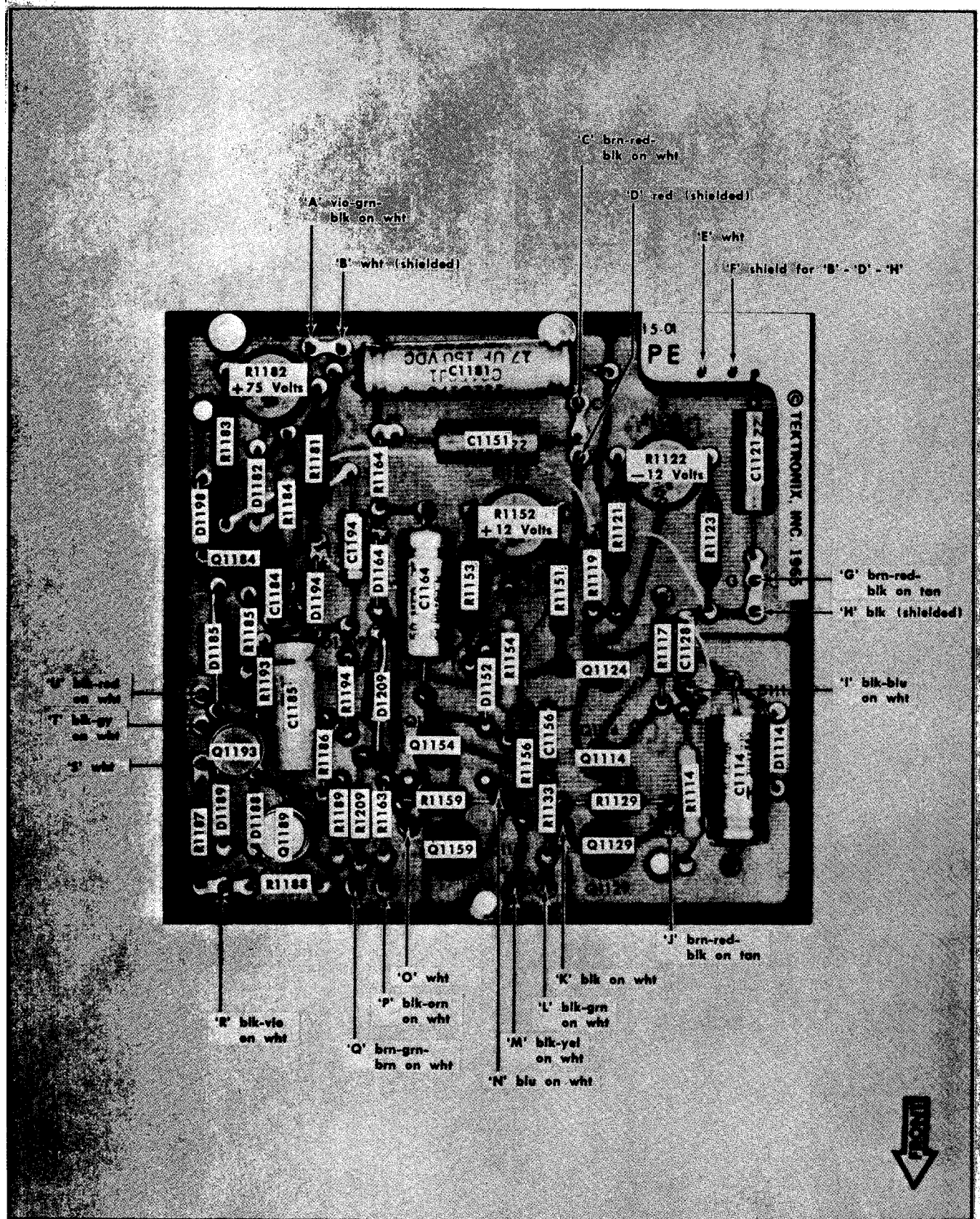
Fig. 4-16. Low Voltage Regulator circuit board.
