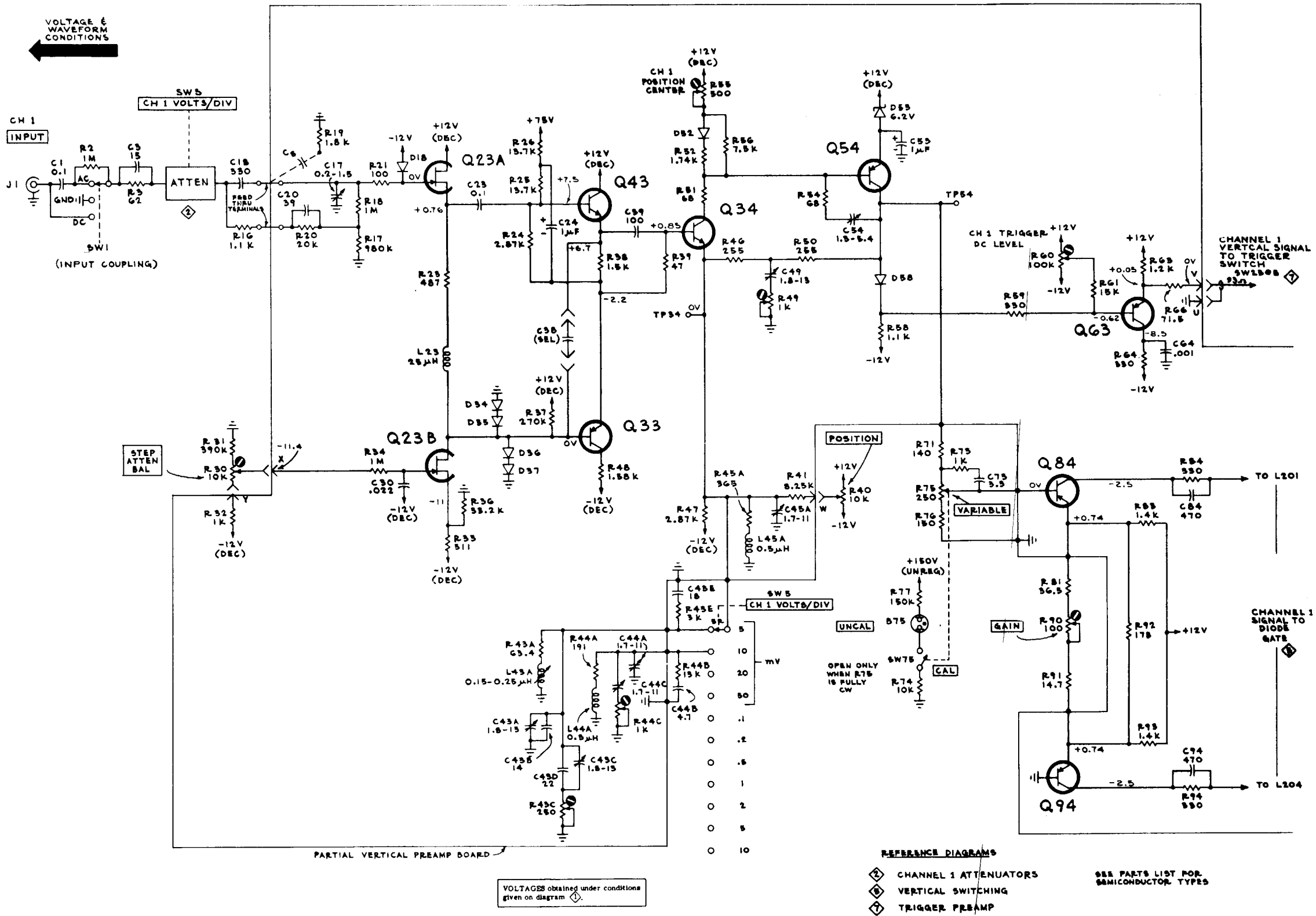
FIG. F0-11. CHANNEL 1 VERTICAL PREAMP (S/N 20,000 & UP)
