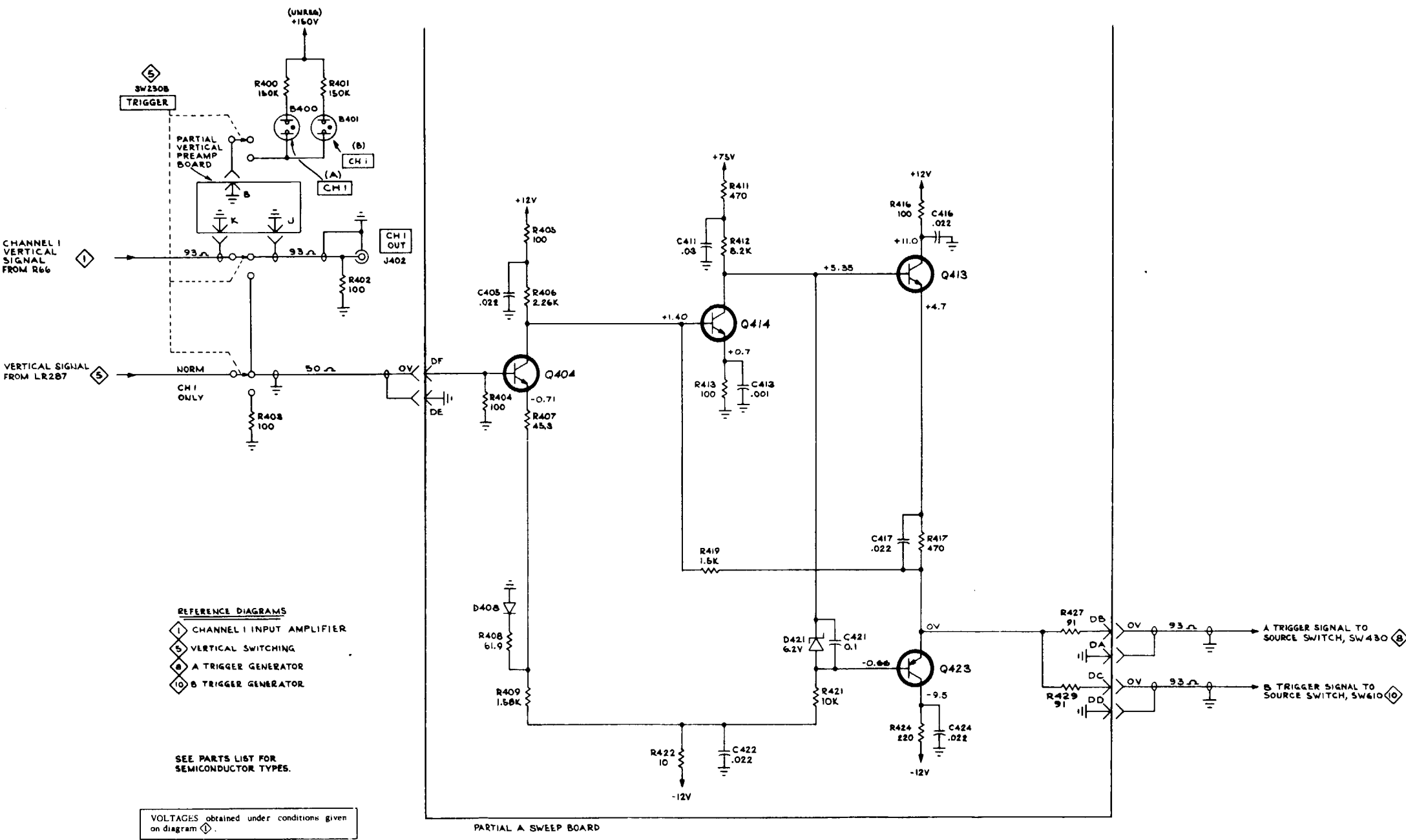
FIG. FO-17 TRIGGER PREAMP (S/N 20,000 & UP)
