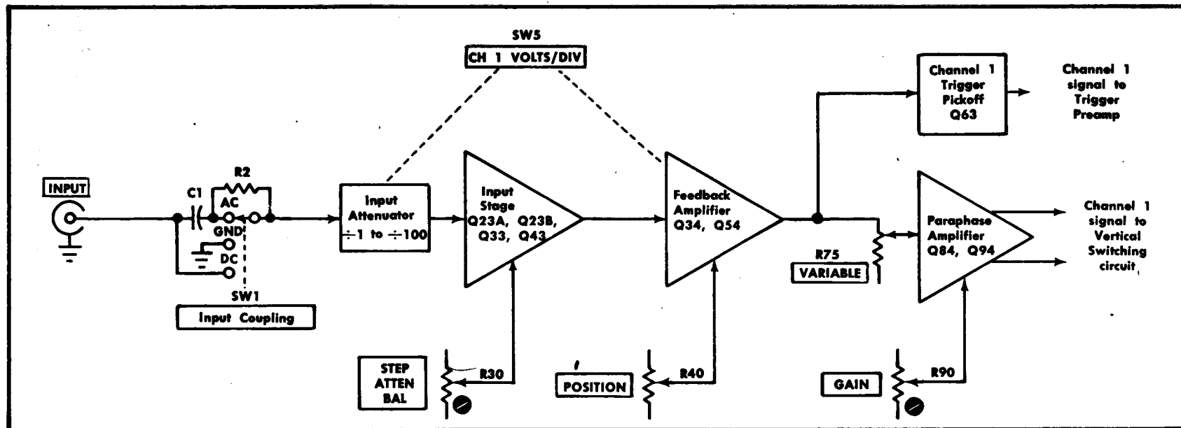
Fig. 3-2. Channel 1 Vertical Preamp detailed block diagram.
