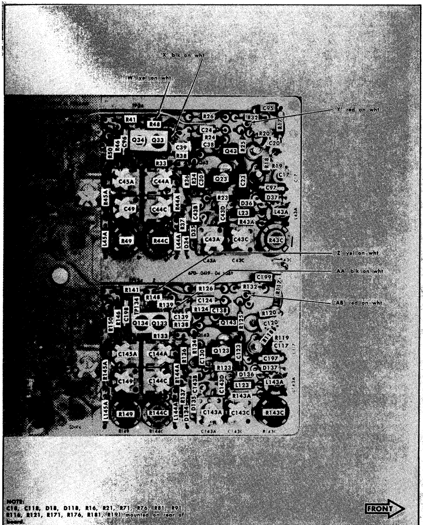
Fig. 4-10. Partial Vertical Preamp circuit board. Partial Vertical Preamp circuit shown.
