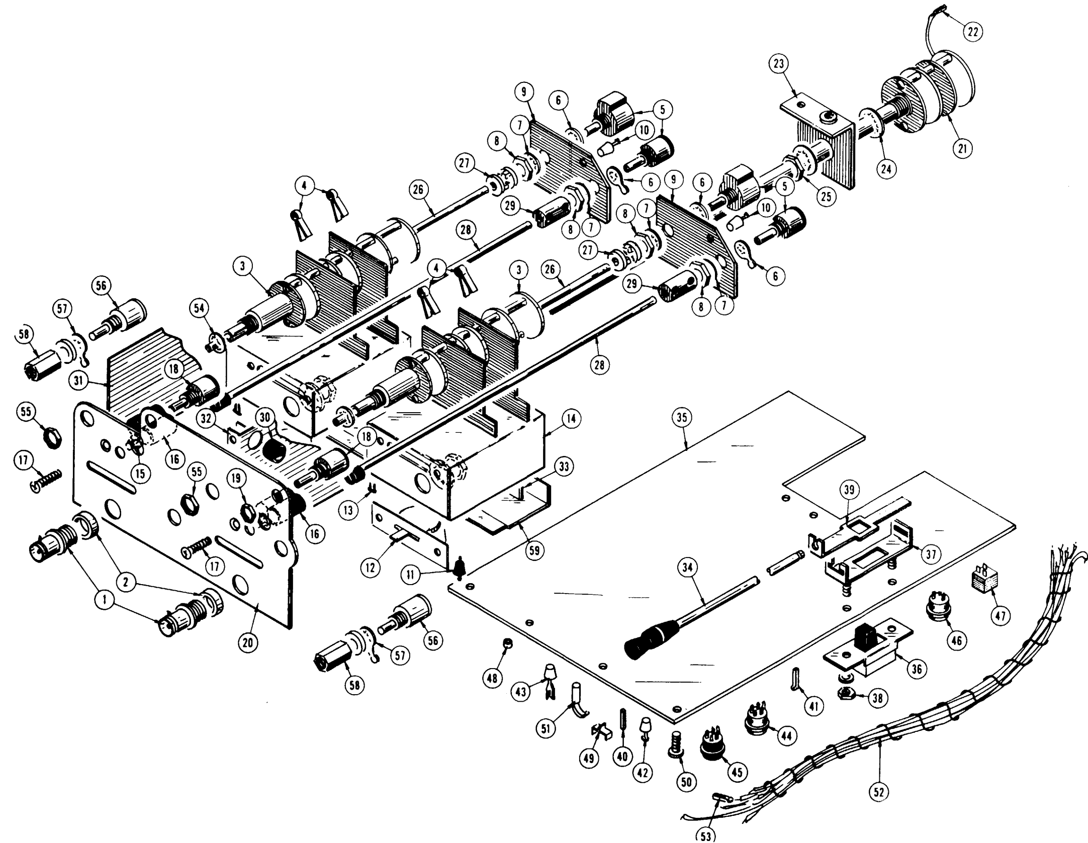
FIG. F0-2 ATTENUATOR PREAMPLIFIER ASSEMBLY
