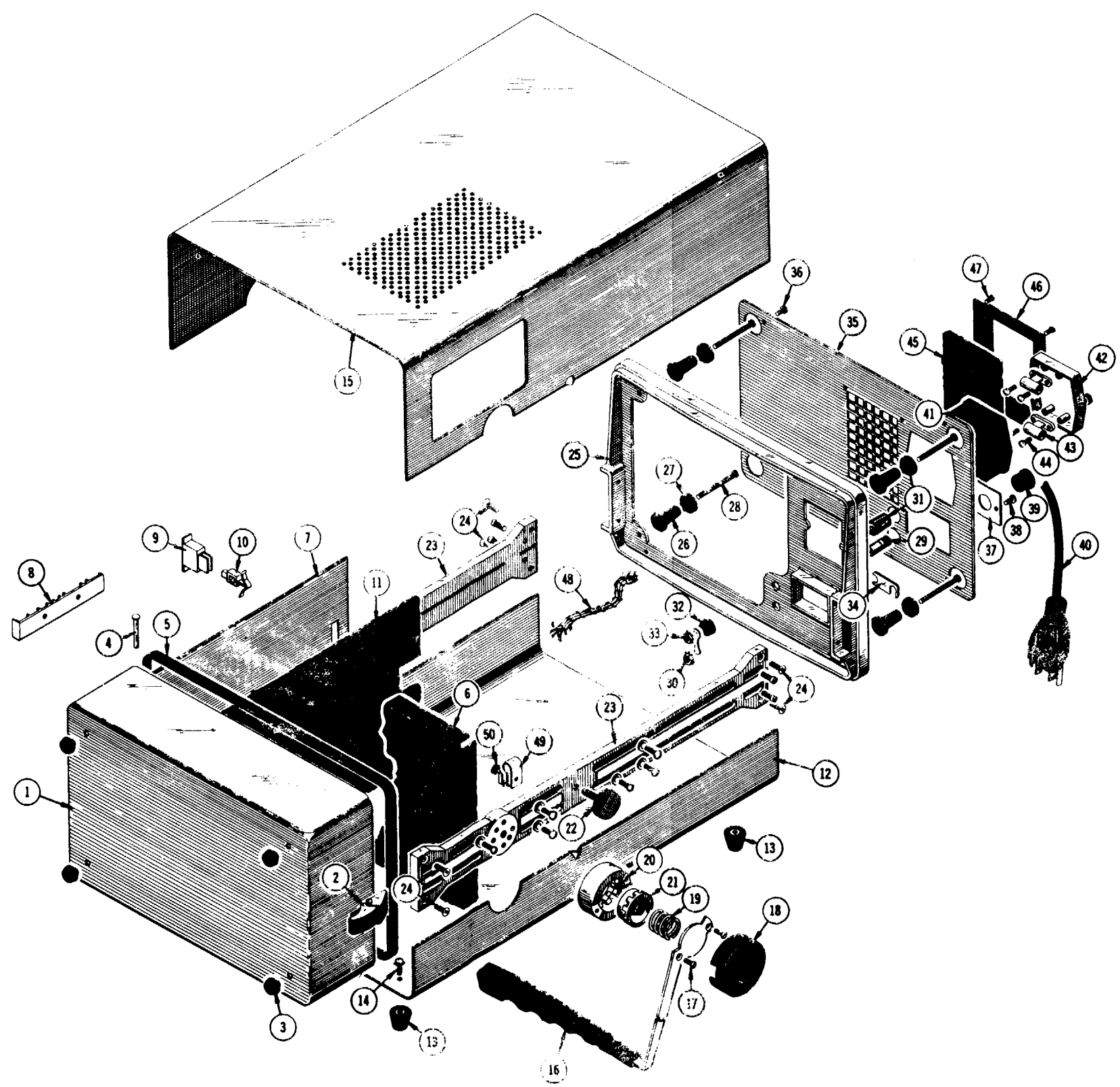
FIG. F0-7 FRAME & CABINET
