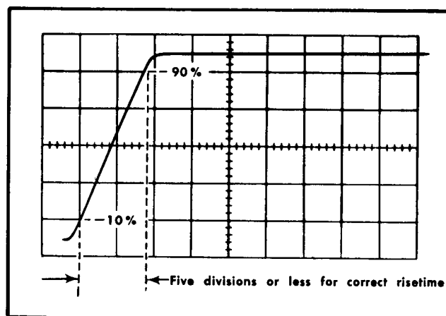
Fig. 5-30. Typical CRT display when checking calibrator risetime.
