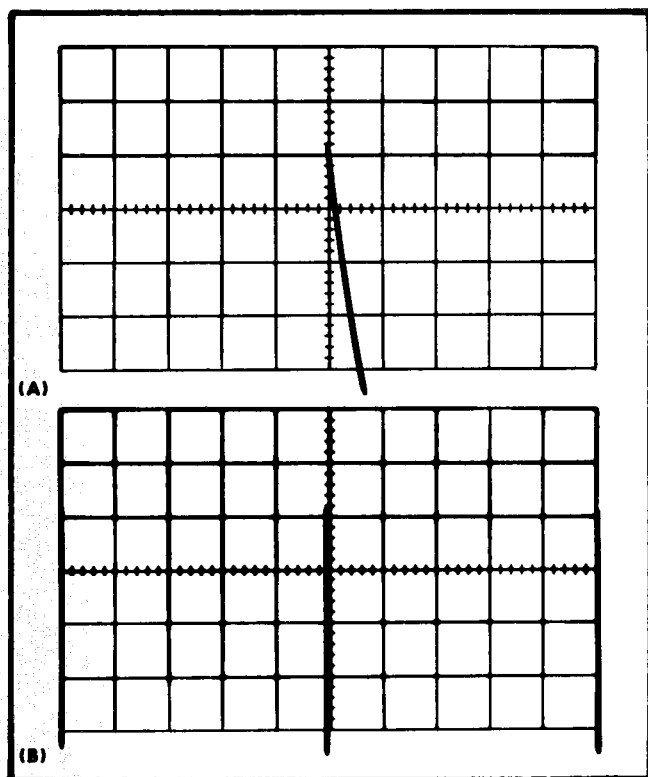
Fig. 5-21. Typical CRT display showing correct magnifier registration. (A) MAG switch set to X10, (B) MAG switch set to OFF.
