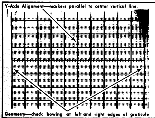
Fig. 5-1. Typical CRT display showing good geometry and Y-axis alignment.
