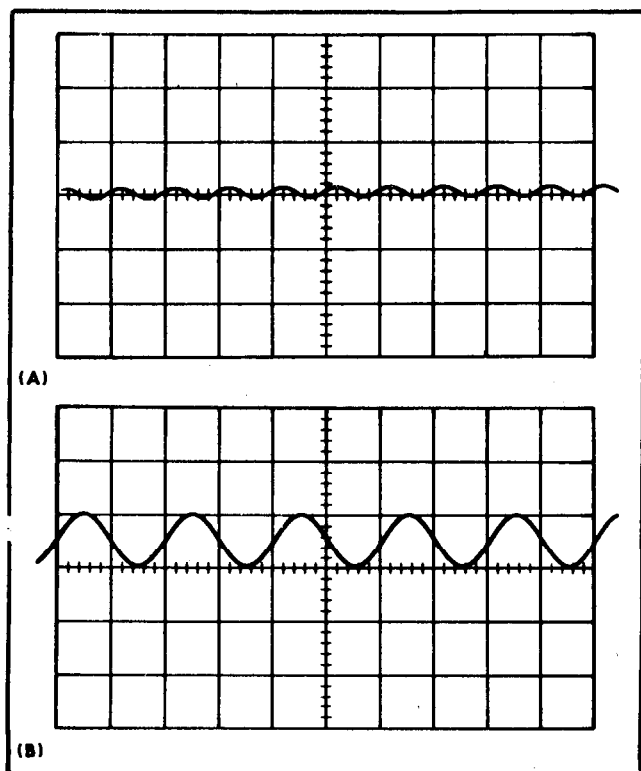
Fig. 6-31. (A) Typical CRT display when checking internal 10 megahertz triggering, (B) typical CRT display when checking internal 50 megahertz triggering.
