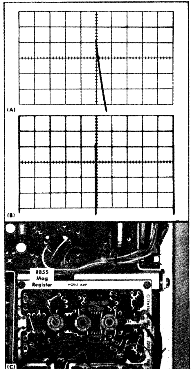
Fig. 6-41. Typical CRT display showing correct magnifier register. (A) MAG switch to \times 10 , (B) MAG switch set to OFF, (C) location of Mag Register adjustment (B Sweep circuit board).
