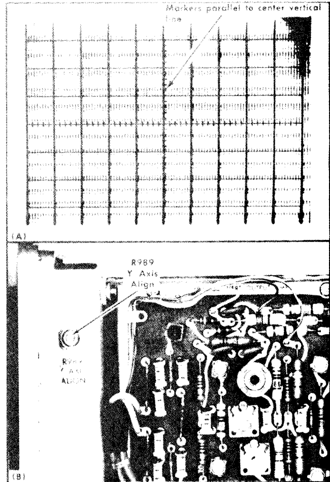
Fig. 6-12. (A) Typical CRT display showing correct Y-axis alignment, (B) location of Y Axis Align adjustment (left side).
