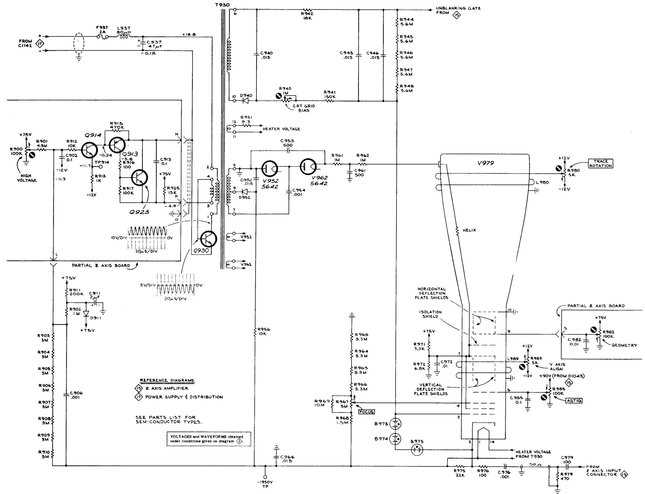
FIG. FO-26. CRT CIRCUIT (S/N 20,000 & UP)
