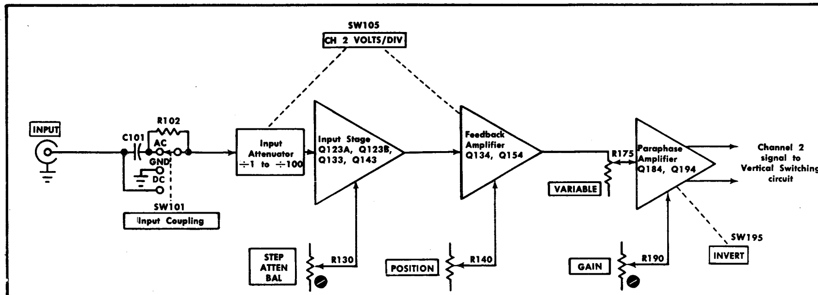
Fig. 3-3. Channel 2 Vertical Preamp detailed block diagram.
