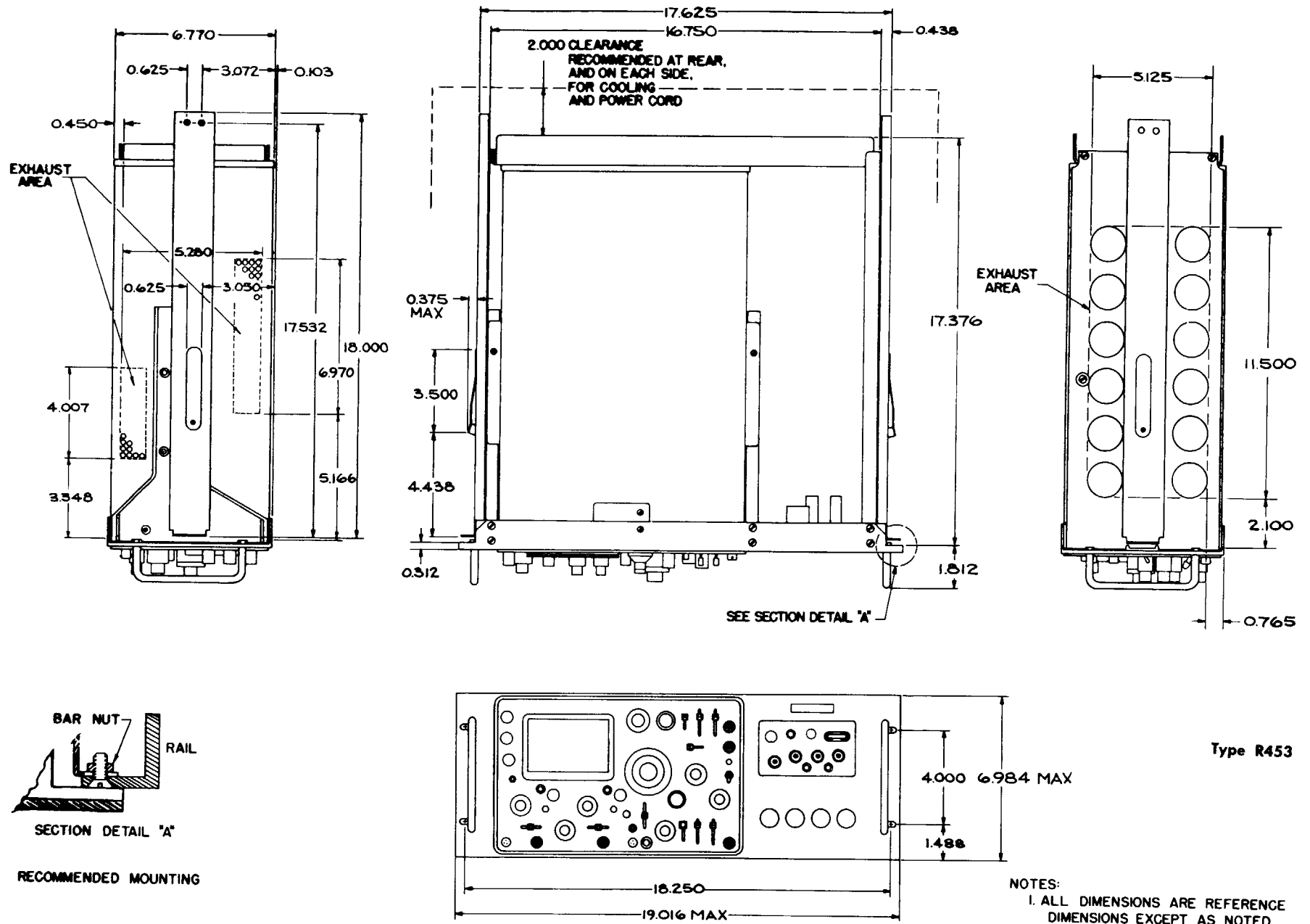
FIGURE 10-14. DIMENSIONAL DRAWING
