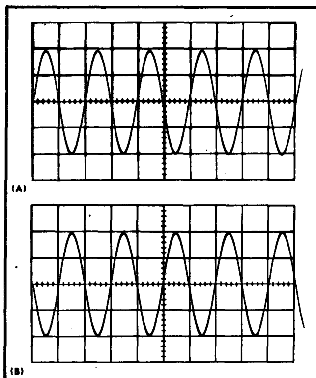
Fig. 6-36. Typical CRT display when checking slope switch operation. (A) SLOPE switch set to +, (B) SLOPE switch set to -.
