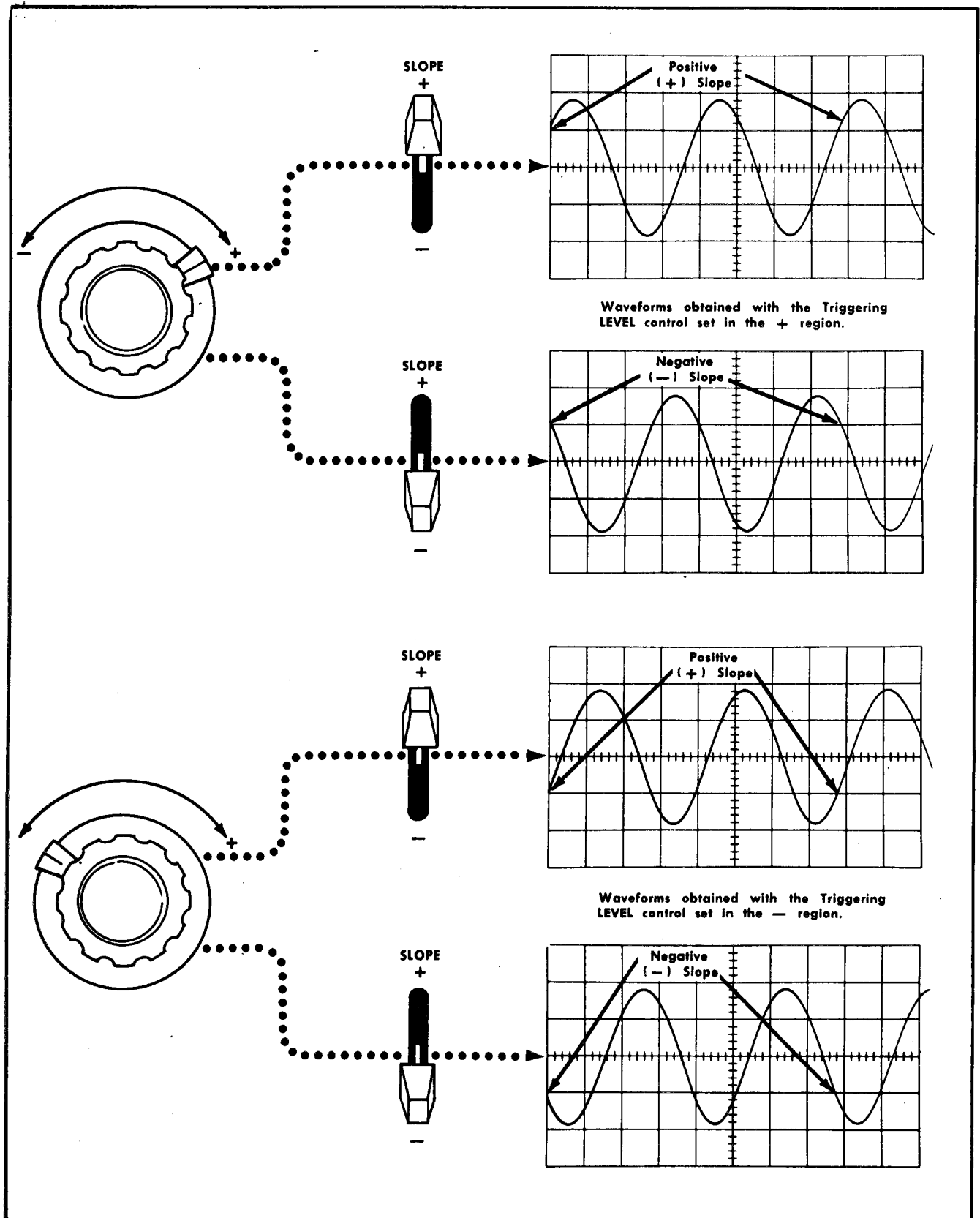
Fig. 2-8. Effects of Triggering LEVEL control and SLOPE switch.
