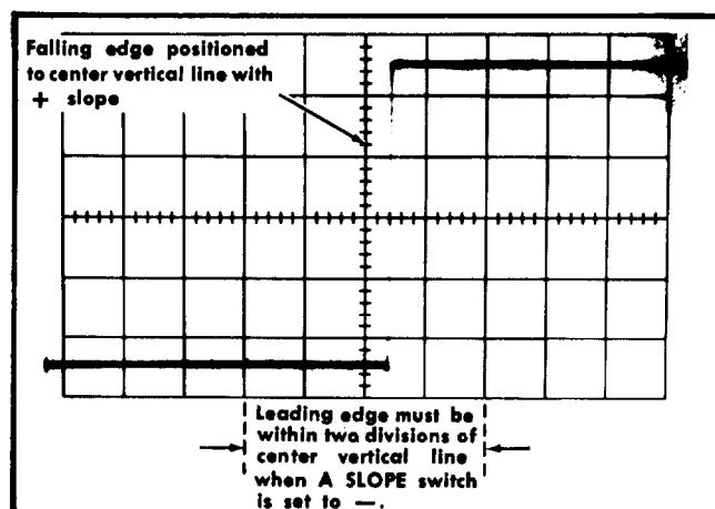
Fig. 6-57. Typical CRT display when checking calibrator duty cycle.
