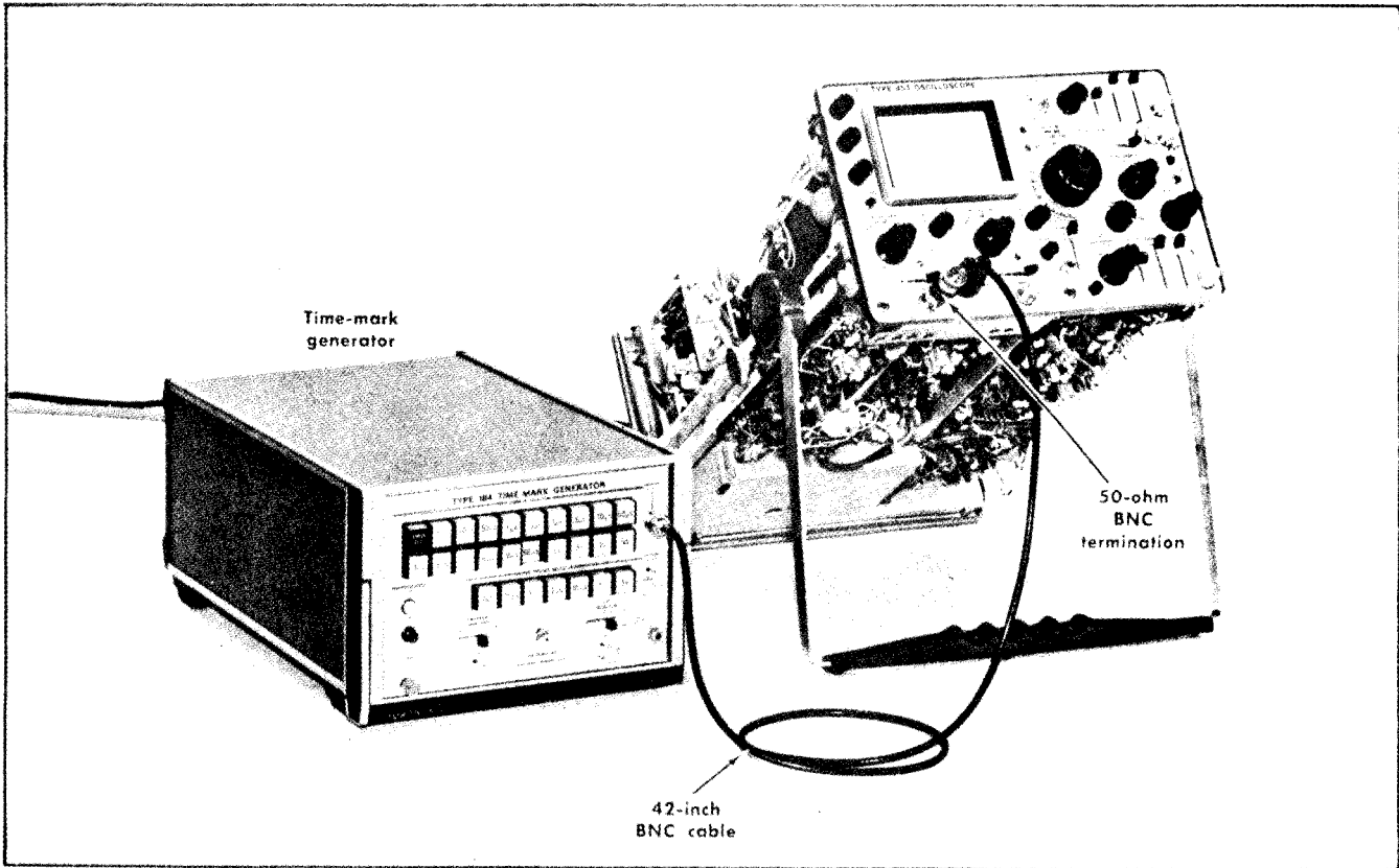
Fig. 6-37. Initial test equipment setup for steps 41 through 60.
