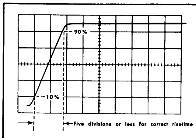
Fig. 6-58. Typical CRT display when checking Calibrator risetime.
