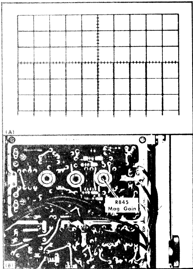
Fig. 6-40. (A) Typical CRT display showing correct magnified gain; (B) location of Mag Gain adjustment (B Sweep circuit board).
