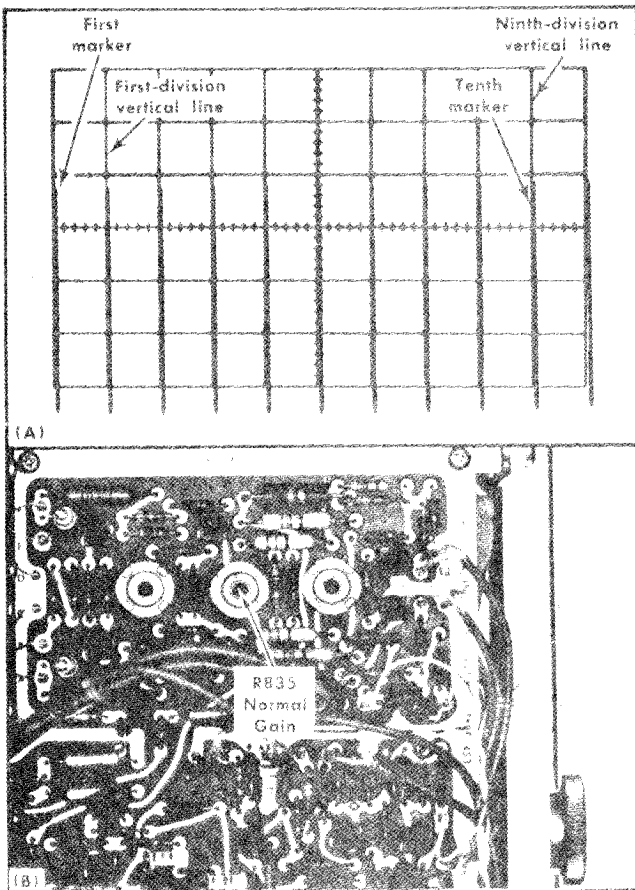
Fig. 6-39. (A) Typical CRT display showing correct normal gain; (B) location of Normal Gain adjustment (B Sweep circuit board).
