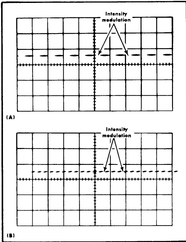
Fig. 5-33. (A) Typical CRT display when checking Z-axis operation at 50 kilohertz, (B) typical CRT display when checking Z-axis operation at 50 megahertz.
