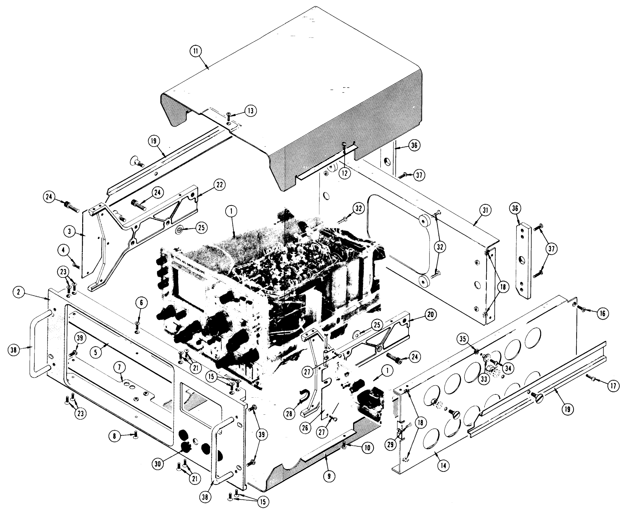
FIG. F0-8 R453 MECHANICAL PARTS
