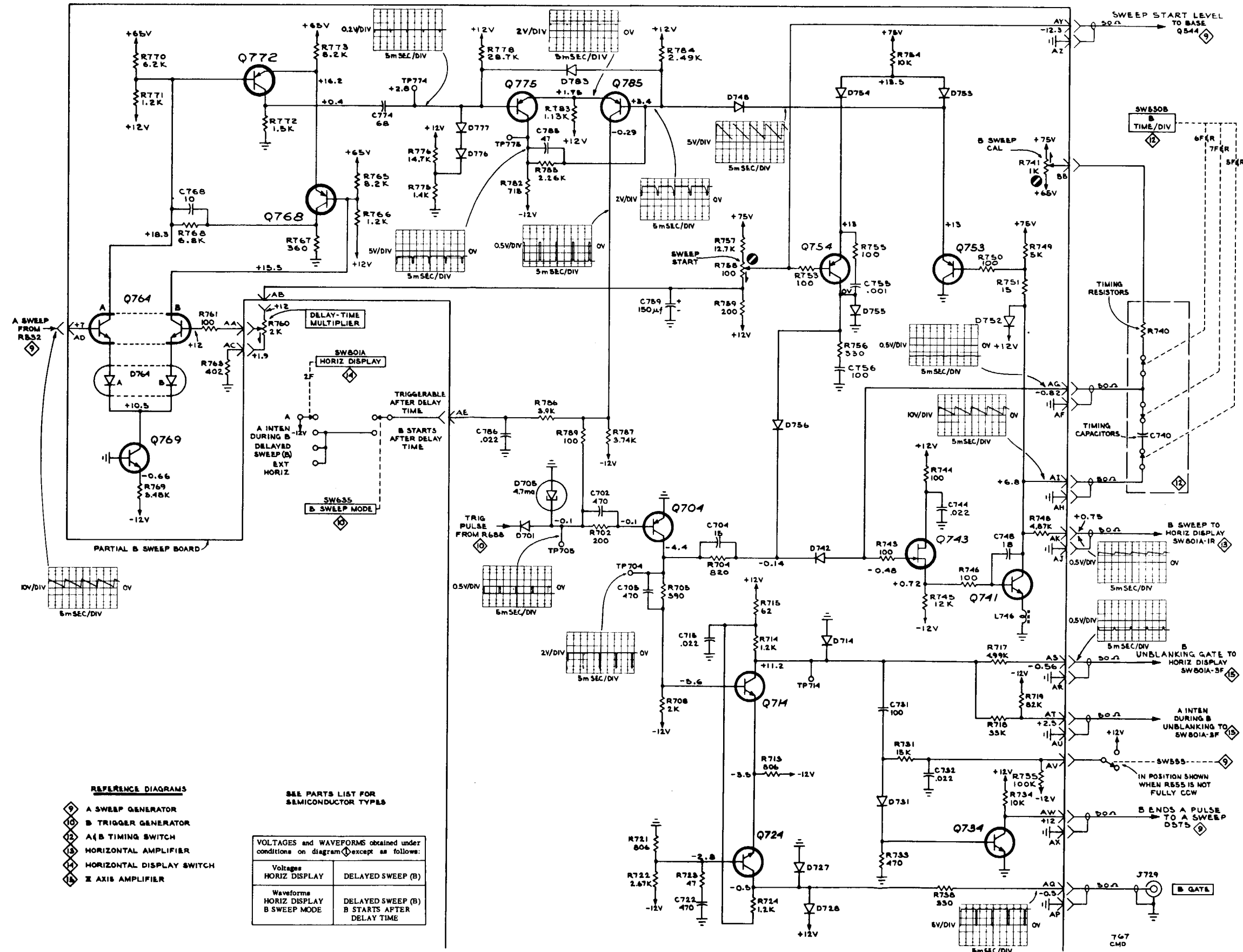
TYPE 453 OSCILLOSCOPE
