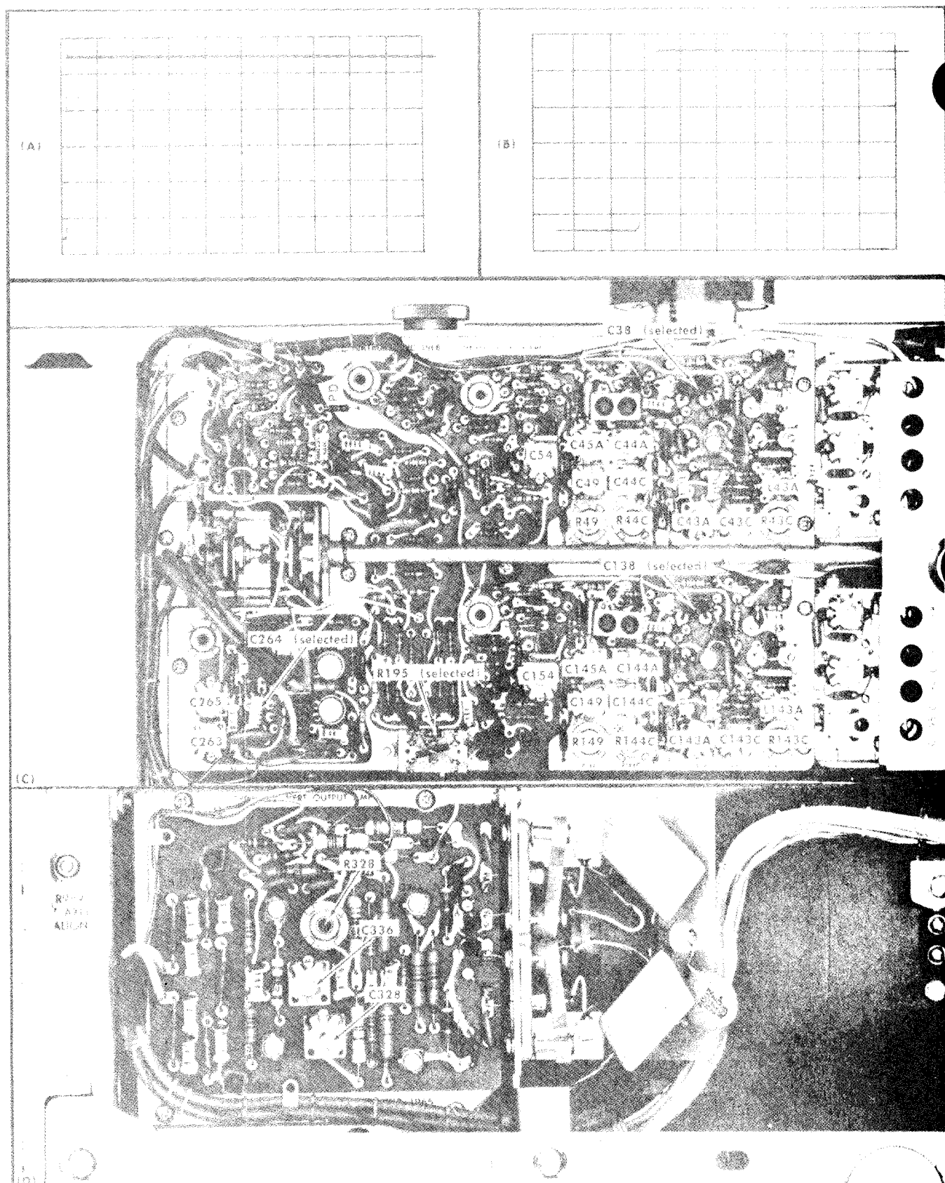
Fig. 6-2.2. (A) Typical CRT display showing correct high-frequency compensation (0.5 microseconds/division) ; (B) typical CRT display showing correct high-frequency compensation (10 nanoseconds/division) ; (C) location of high-frequency compensation adjustments and selected components (Vertical Preamp circuit board) ; (D) location of R328, C328 and C336 (Vertical Output Amplifier circuit board) .
