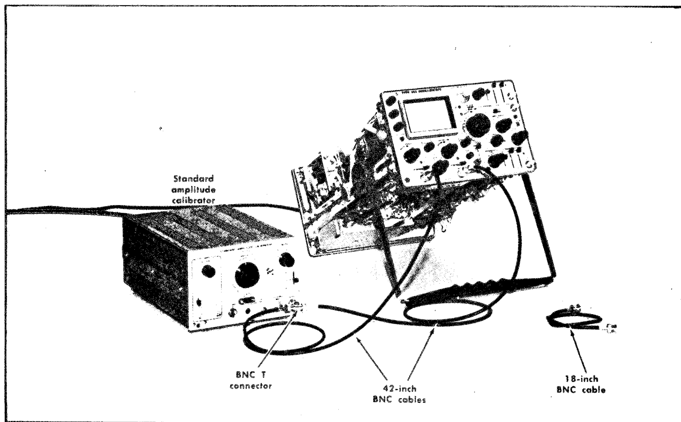
Fig. 6-16. Initial test equipment setup for steps 13 through 21.
