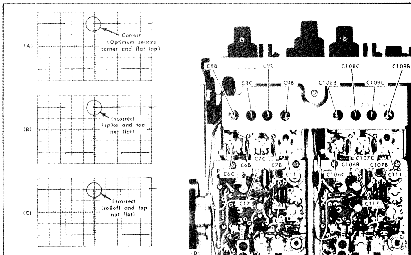
Fig. 6-21. (A) Typical CRT display showing correct compensation; (B) and (C) incorrect compensation; (D) location of variable capacitors (bottom view).
