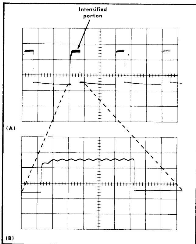
Fig. 2-12. (A) A INTEN DURING B display (DELAY-TIME MULTIPLIER, 2.95; A TIME/DIV, .5 ms; B TIME/DIV, 50 \mu s), (B) DELAYED SWEEP (B) display.
