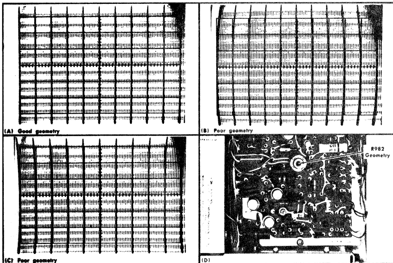
6 - 13 . (A) Typical CRT display showing good geometry; (B) and (C) poor geometry; (D) Location of Geometry adjustment (Z Axis Amplifier circuit board).
