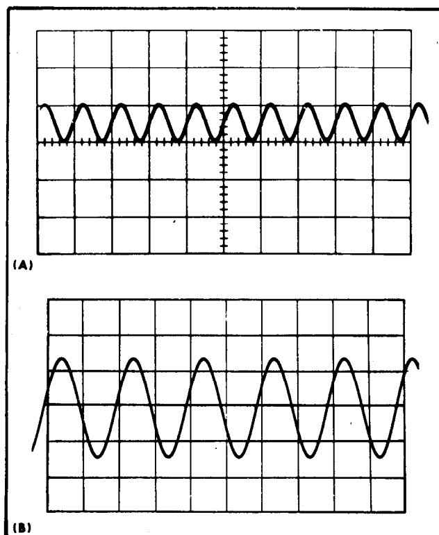
Fig. 6-32. (A) Typical CRT display when checking external 10 megahertz triggering, (B) typical CRT display when checking external 50 megahertz triggering.
