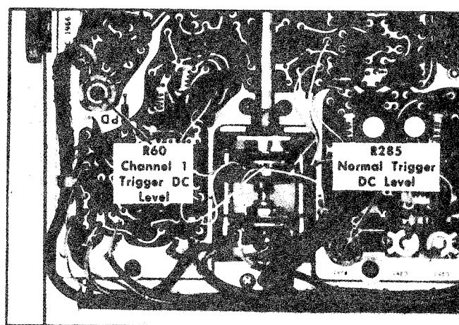
Fig. 6-30. Location of Channel 1 Trigger and Normal Trigger DC level (Vertical Preamp circuit board).
