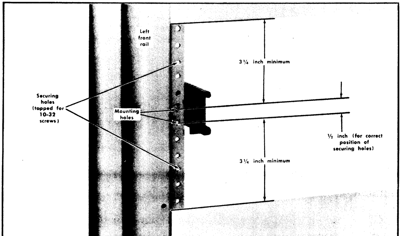
Fig. 10-6. Locating the mounting holes for the left stationary section. Same dimensions apply to right stationary section.
