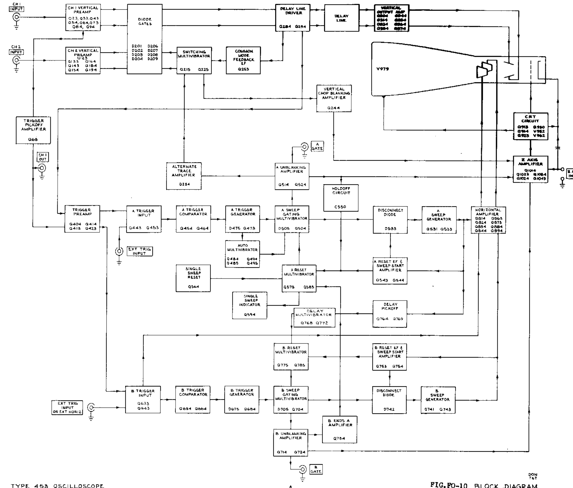
TYPE 453 OSCILLOSCOPE
