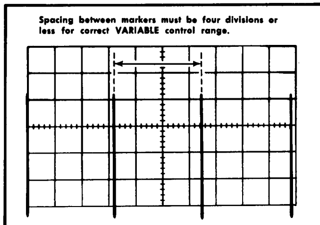
Fig. 5-23. Typical CRT display when checking A and B VARIABLE control range.
