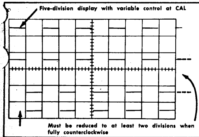
Fig. 6-18. Typical CRT display showing adequate Channel 1 and 2 VARIABLE control range (double exposure).
