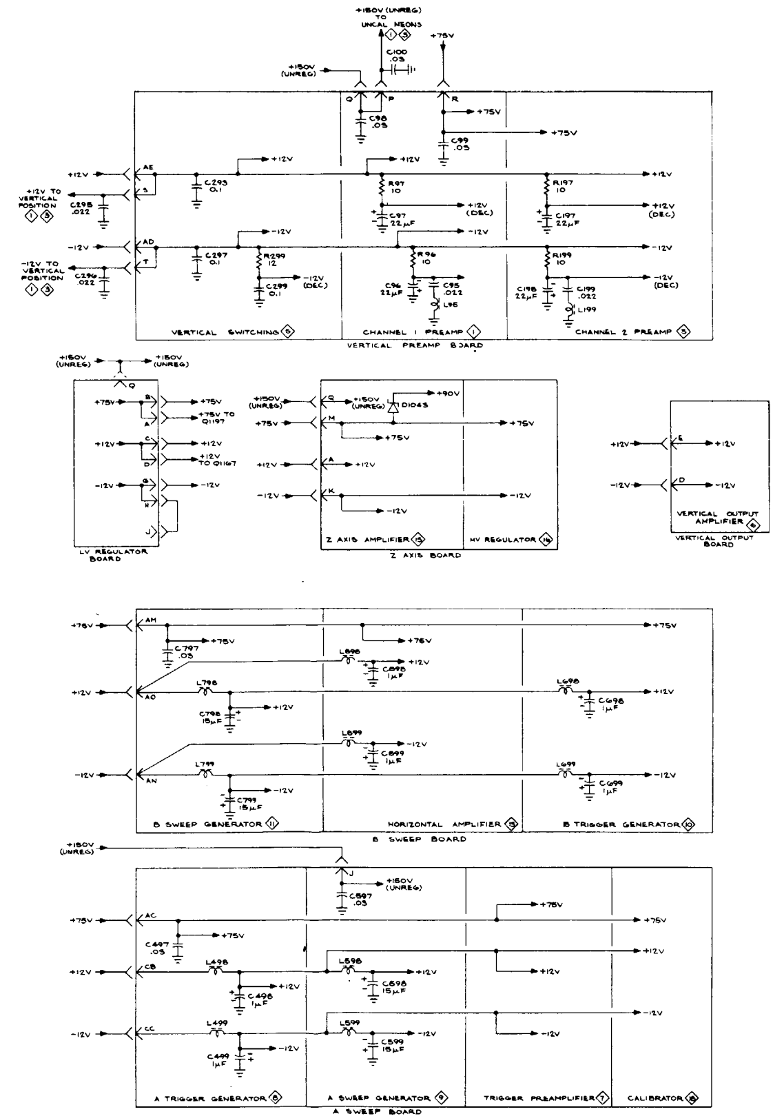
FIG. F0-27. POWER SUPPLY & DISTRIBUTION (S/N 20,000 & UP)
