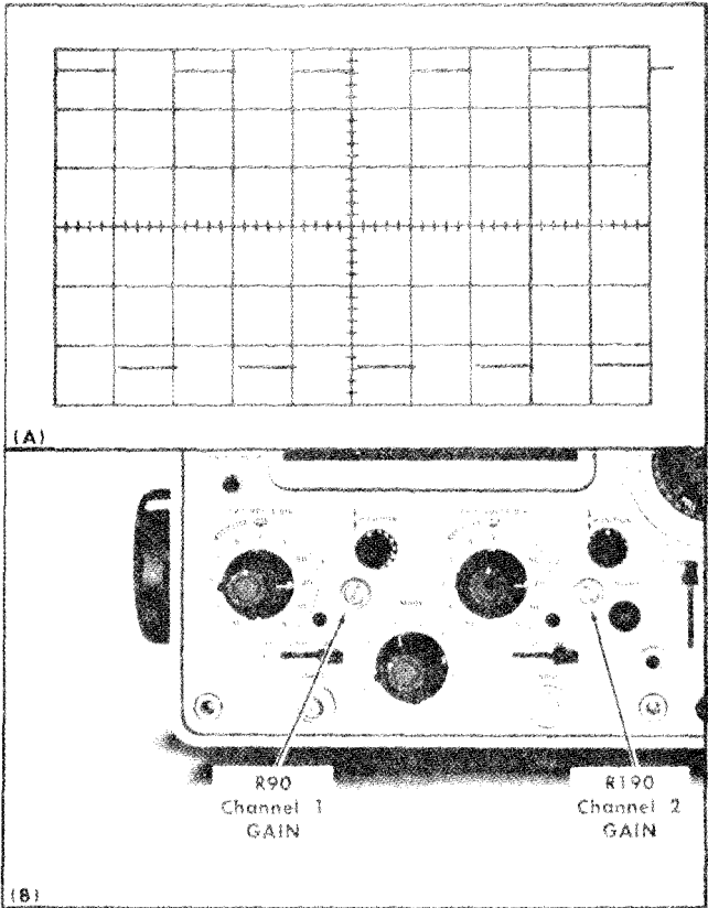
Fig. 6-17. (A) Typical CRT display showing correct gain adjustments; (B) location of Channel 1 and 2 GAIN adjustments (front panel).
