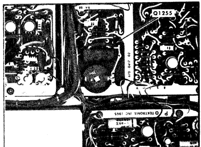
Fig. 6-5. Location of Q1255 (Calibrator section of A Sweep circuit board).
