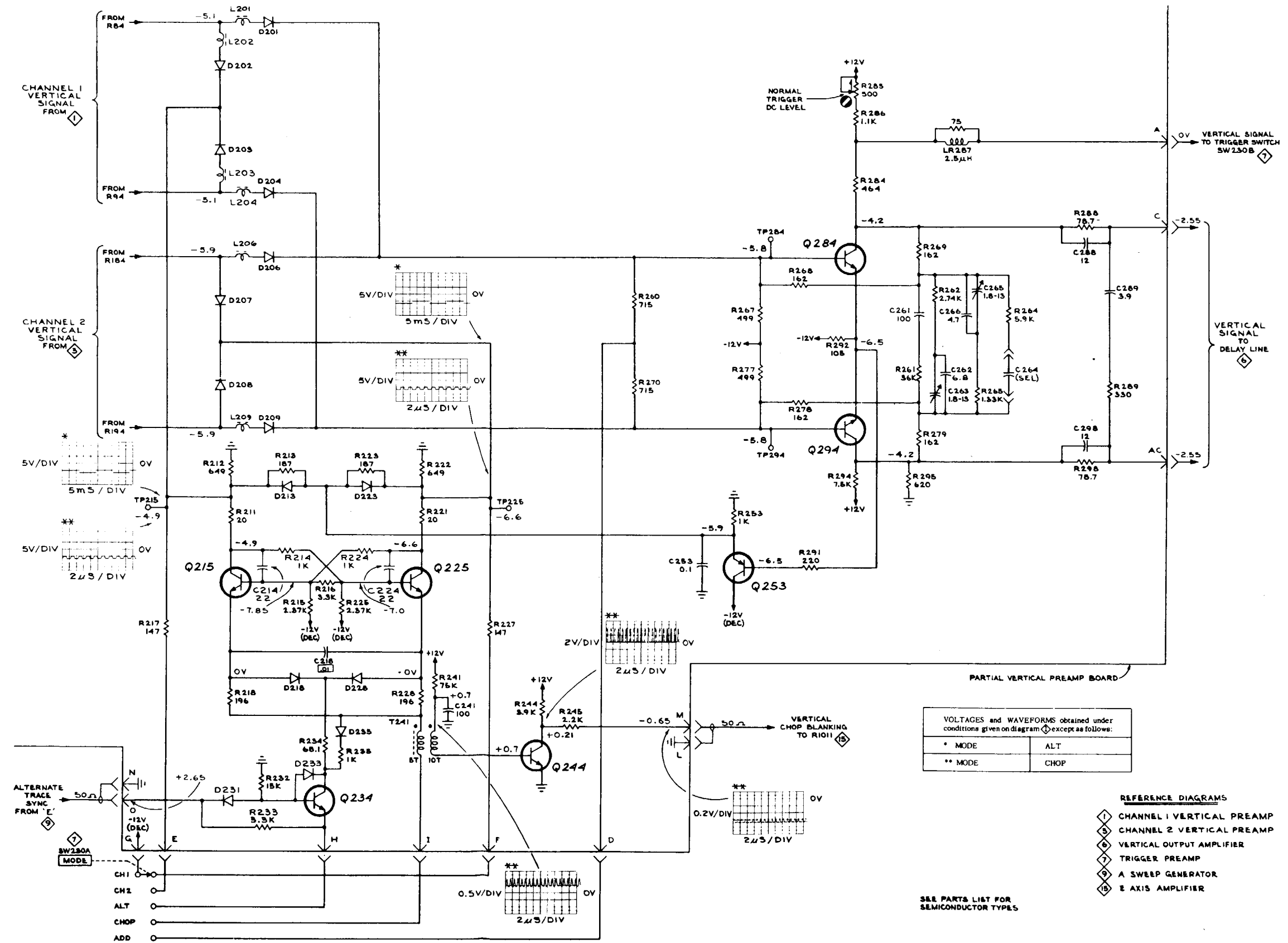
TYPE 453 OSCILLOSCOPE
