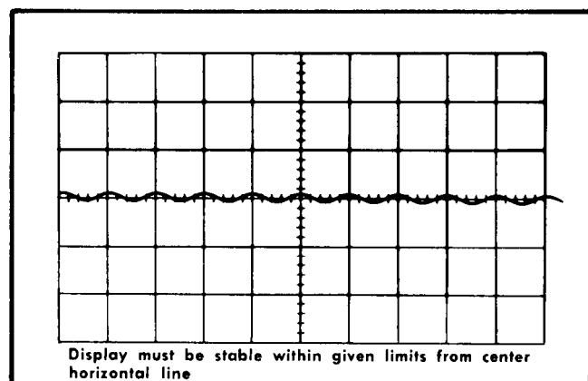
Fig. 5-10. Typical CRT display when checking trigger level centering.
