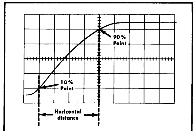
Fig. 2-18. Measuring risetime.
