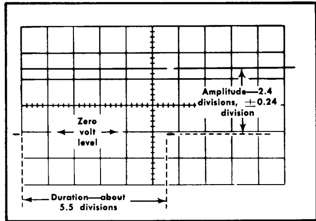
Fig. 5-34. Typical test oscilloscope display when checking A and B GATE output amplitude and duration (vertical deflection factor, five volts/division; sweep rate, two milliseconds/division).
