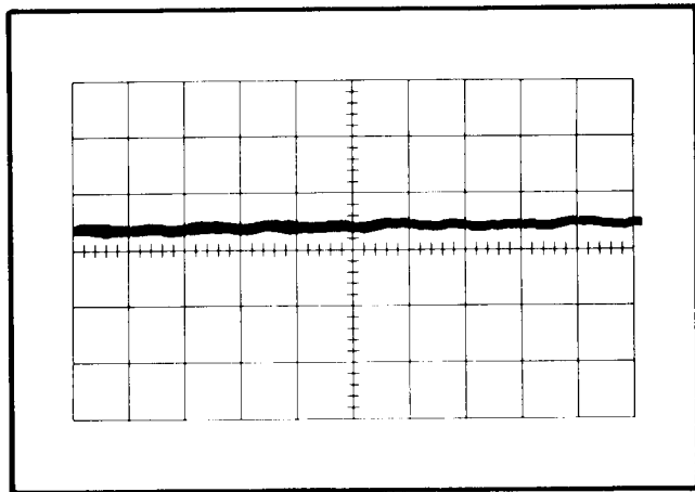
Fig. 6-8. Typical test oscilloscope display of power-supply ripple (60-cycle line). Vertical 0.005 volt/division; sweep rate, five milliseconds/division.
