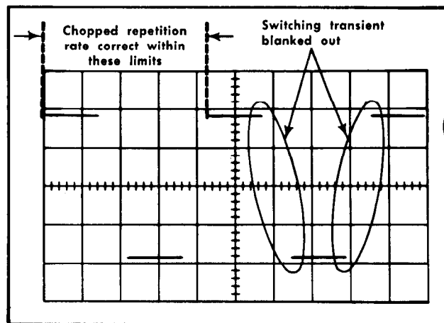
Fig. 6 - 5 4 . Typical CRT display when checking chopped repetition rate and blanking.
