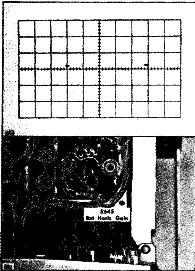
Fig. 6-51. (A) Typical CRT display showing correct external horizontal gain, (B) location of Ext Horiz Gain adjustment (B Sweep circuit board).
