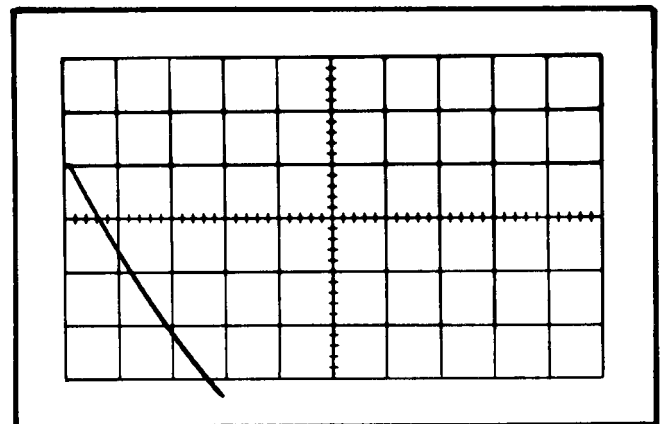
Fig. 5-19. Typical CRT display when checking DELAY-TIME MULTIPLIER dial incremental linearity.
