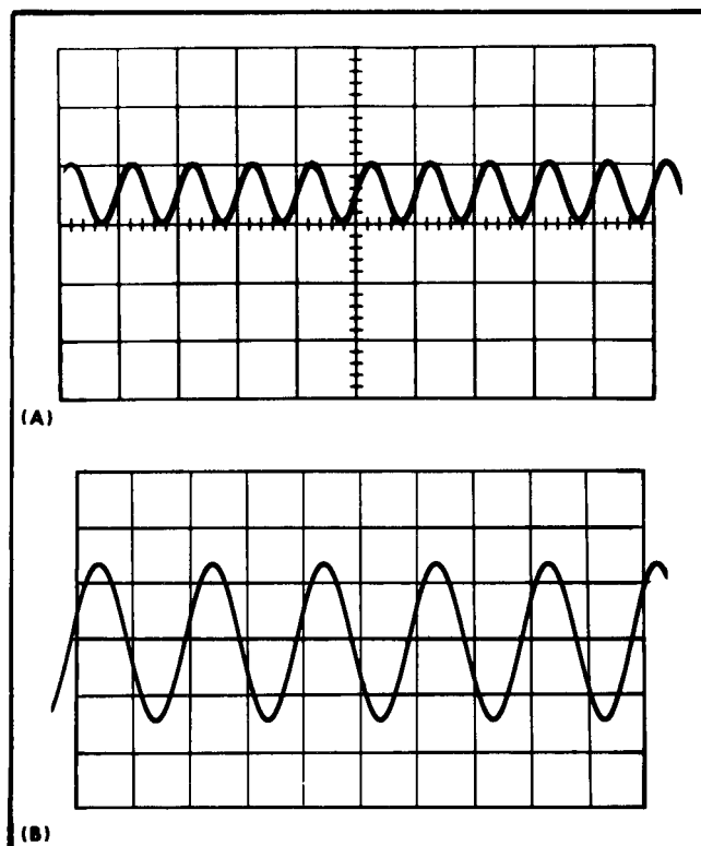
Fig. 5-12. (A) Typical CRT display when checking external 10-megahertz triggering, (B) typical CRT display when checking external 50-megahertz triggering.
