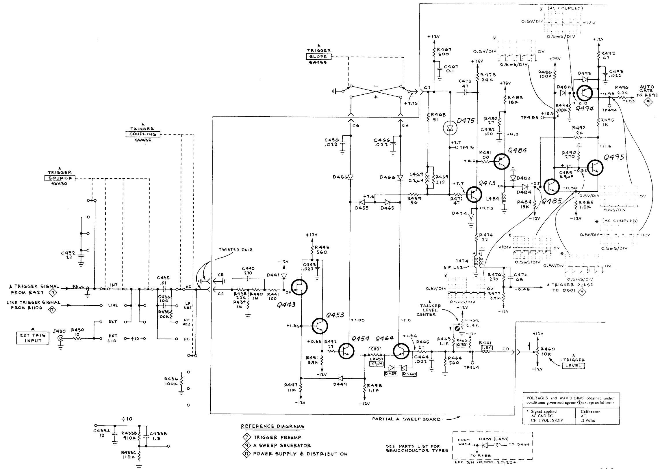
FIG. F0-18 A TRIGGER GENERATOR (S/N 20,000 & UP) 8
