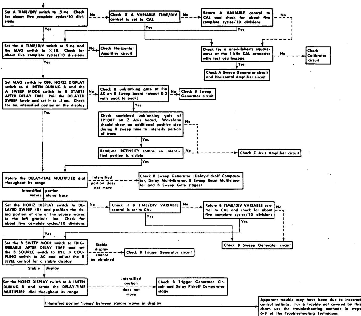
Fig. 4-3. Troubleshooting chart for Type 453.
