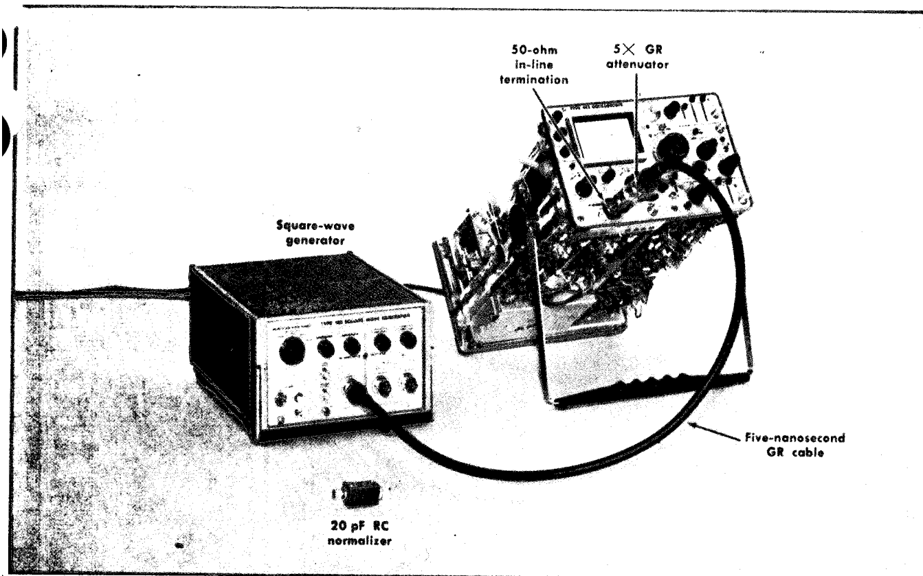
Fig. 6-20. Initial test equipment setup for steps 22 through 24.
