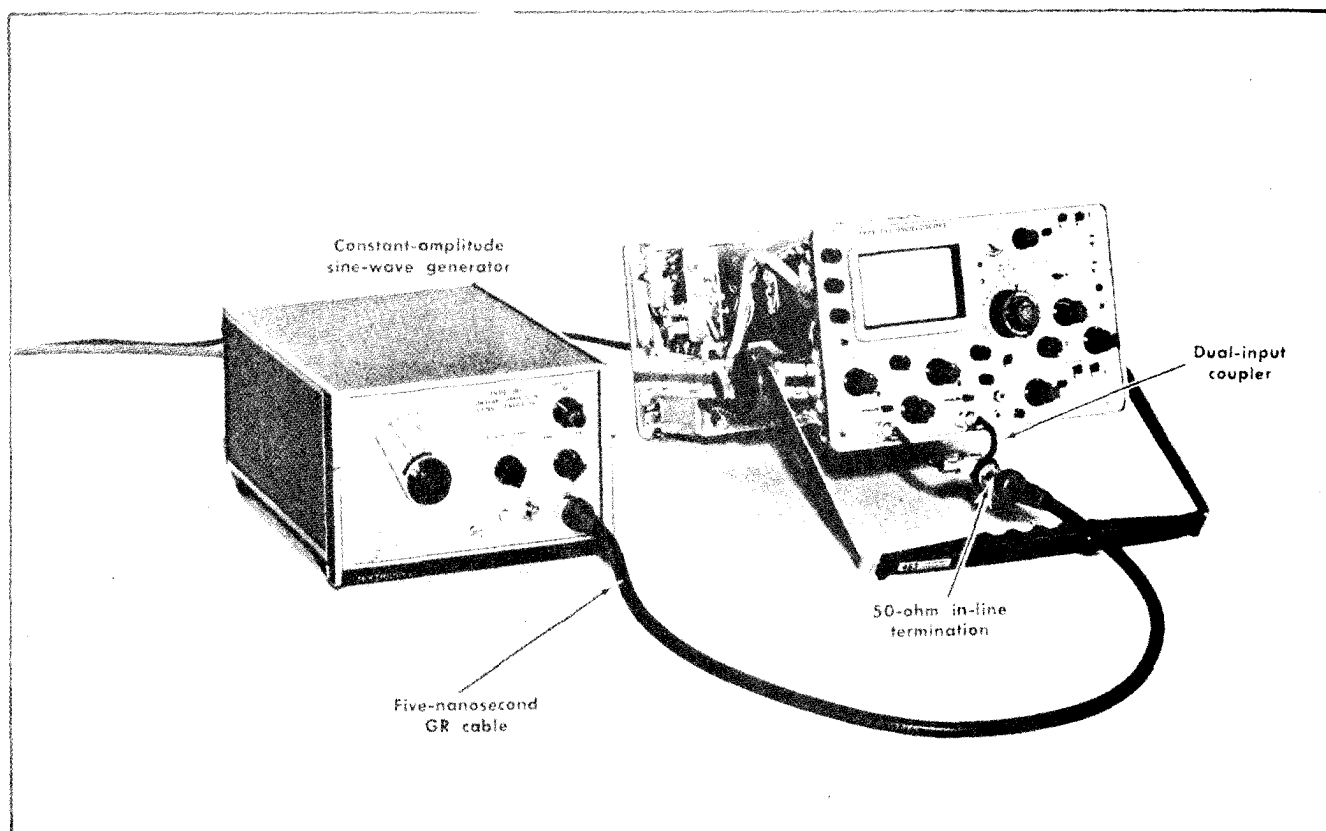
Fig. 6-25. Test equipment setup for steps 28 and 29.
