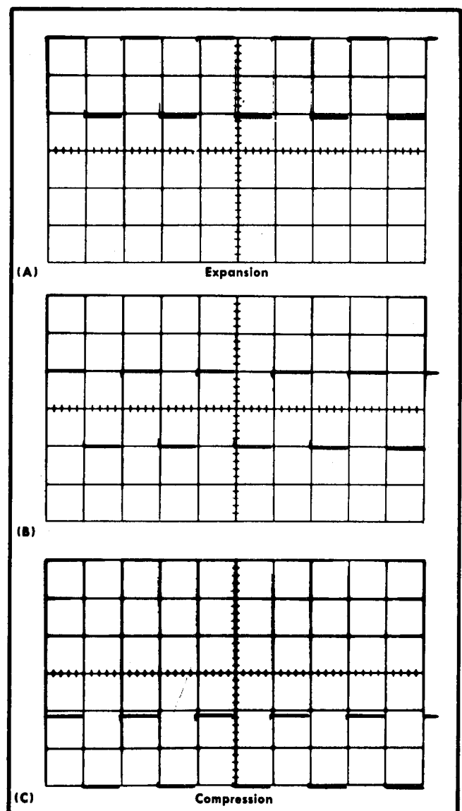
Fig. 6-19. Typical CRT display showing acceptable compression and expansion. (A) Expansion, (B) correct deflection at center of graticule, (C) compression.
