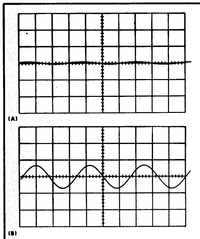
Fig. 6-33. (A) Typical CRT display when checking internal low-frequency triggering at 60 hertz, (B) typical CRT display when checking external low-frequency triggering at 60 hertz.
