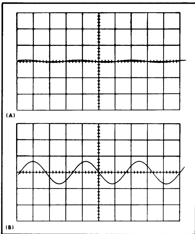
Fig. 5-13. (A) Typical CRT display when checking internal low-frequency triggering at 60 hertz. (B) Typical CRT display when checking external low-frequency triggering at 60 hertz.
