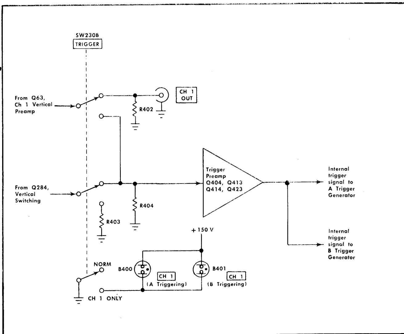
Fig. 3-7. Trigger Preamp detailed diagram
