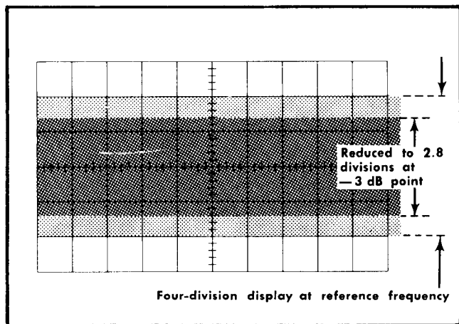
Fig. 5-7. Typical CRT display when checking vertical frequency response (simulated waveform)
