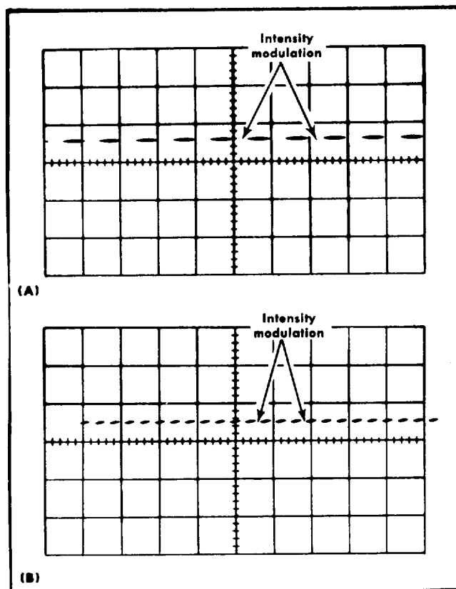
Fig. 6-62. (A) Typical CRT display when checking Z-axis operation at 50 kilohertz, (B) typical CRT display when checking Z-axis operation at 50 megahertz.
