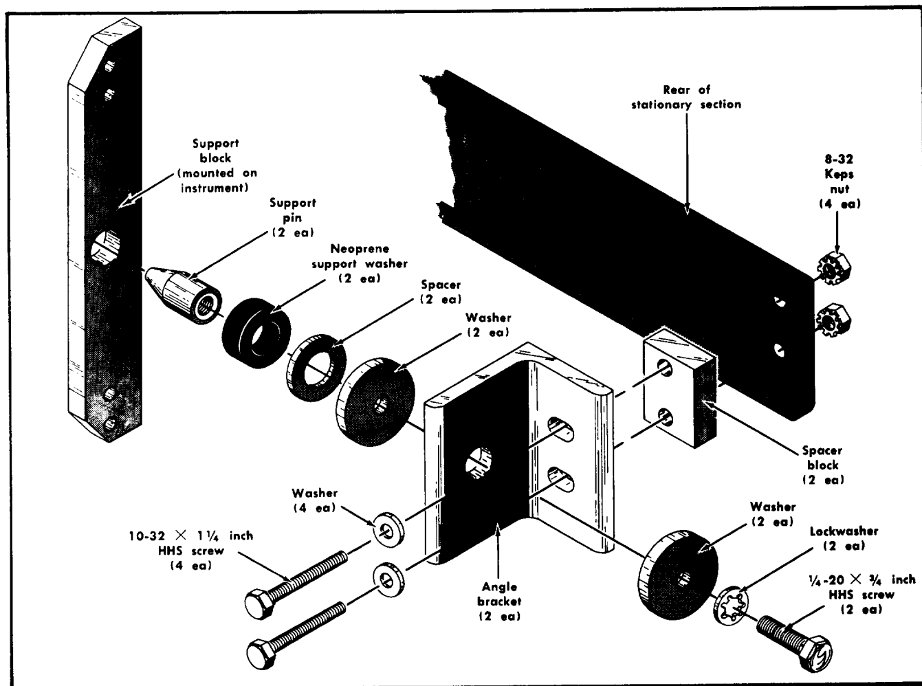
Fig. 10-7. Rear support kit.
