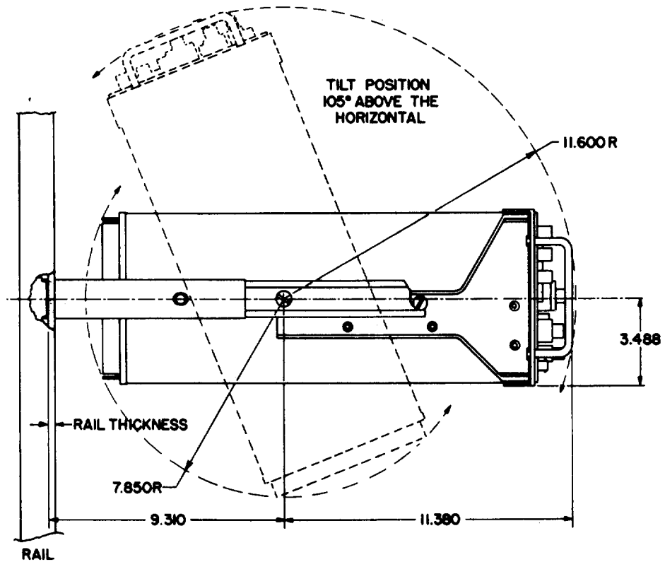
Figure 10-13. Pivoting Dimensions.
