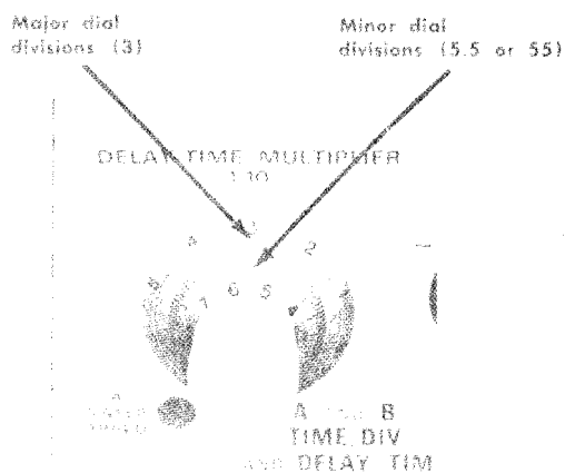
Fig. 2-13. DELAY-TIME MULTIPLIER dial. Reading shown: 3.55.
