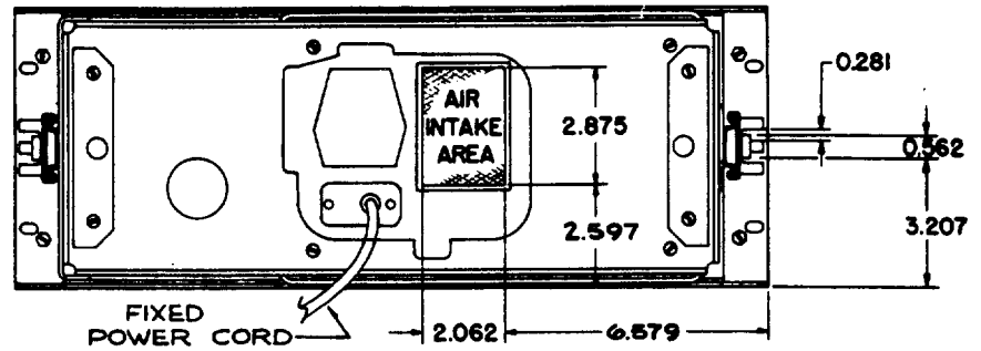
Figure 10-12. REAR VIEW
