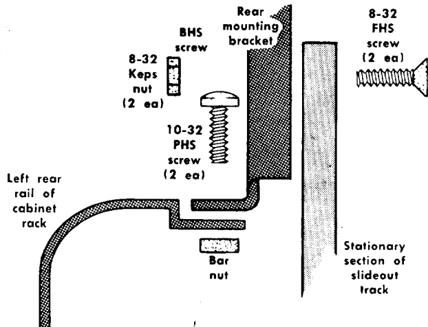
Fig. 10-11. Alternative method of installing the instrument using rear support brackets.
