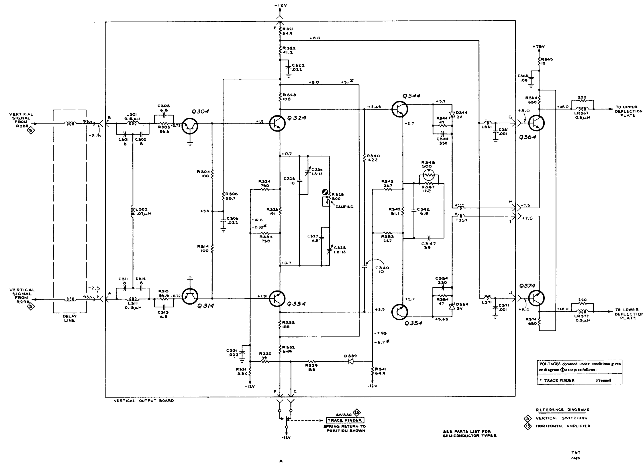
TYPE 453 OSCILLOSCOPE
