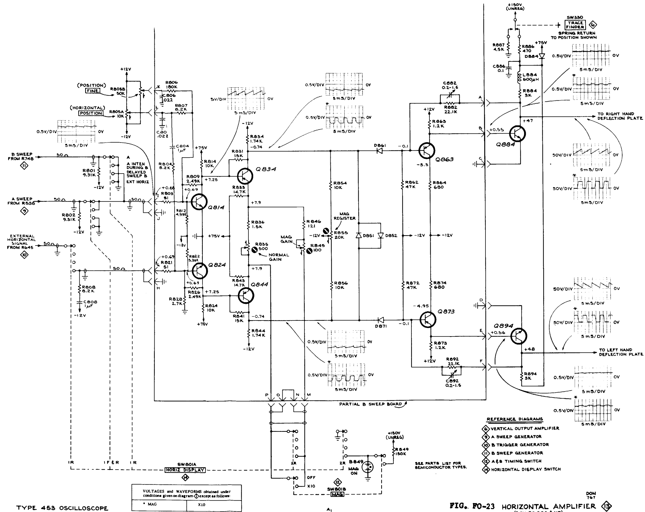
TYPE 453 OSCILLOSCOPE
