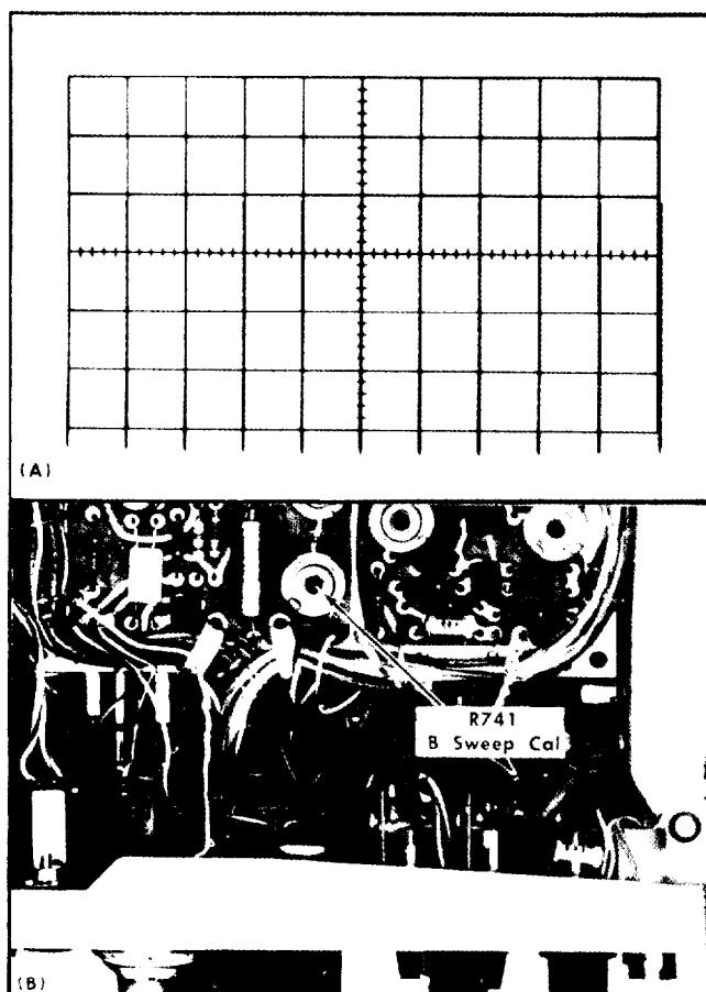
Fig. 6-42. (A) Typical CRT display showing correct B Sweep calibration, (B) location of the B Sweep Cal adjustment of (B Sweep circuit board).
