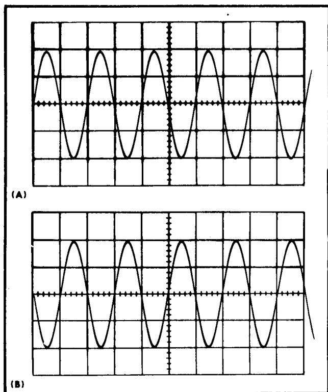
Fig. 5-16. Typical CRT display when checking slope switch operation. (A) SLOPE switch set to +, (B) SLOPE switch set to -.
