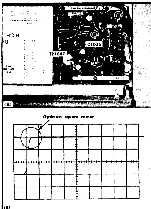
Fig. 6-61. (A) Location of TP1 047 and C1 036, (B) typical test oscilloscope display showing correct adjustment of C1 036 (vertical deflection, 5 volts/division, sweep rate, 0.1 microsecond/division)
