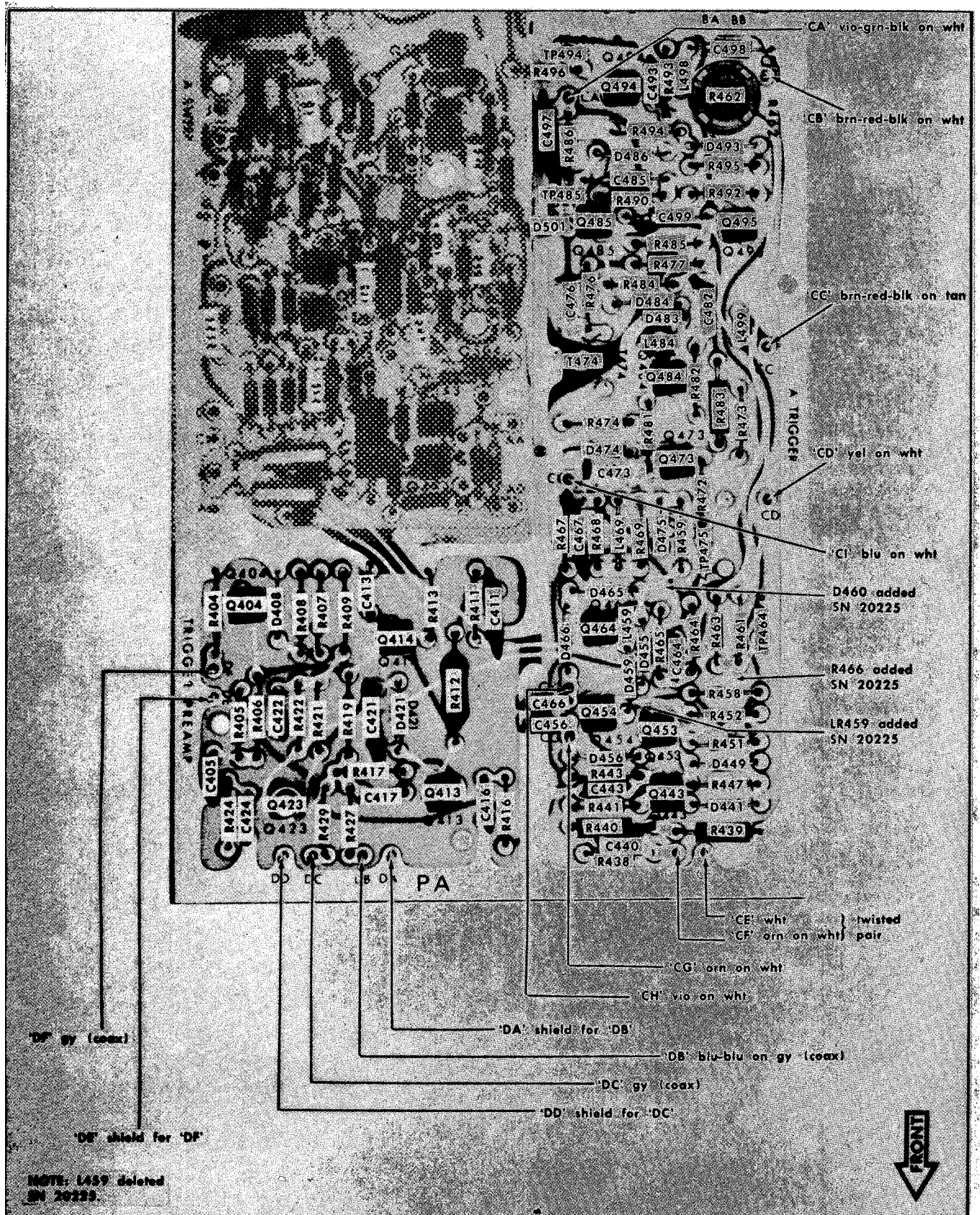
Fig. 4-12. Partial A Sweep circuit board. Trigger Preamp and A Trigger Generator circuits shown.
