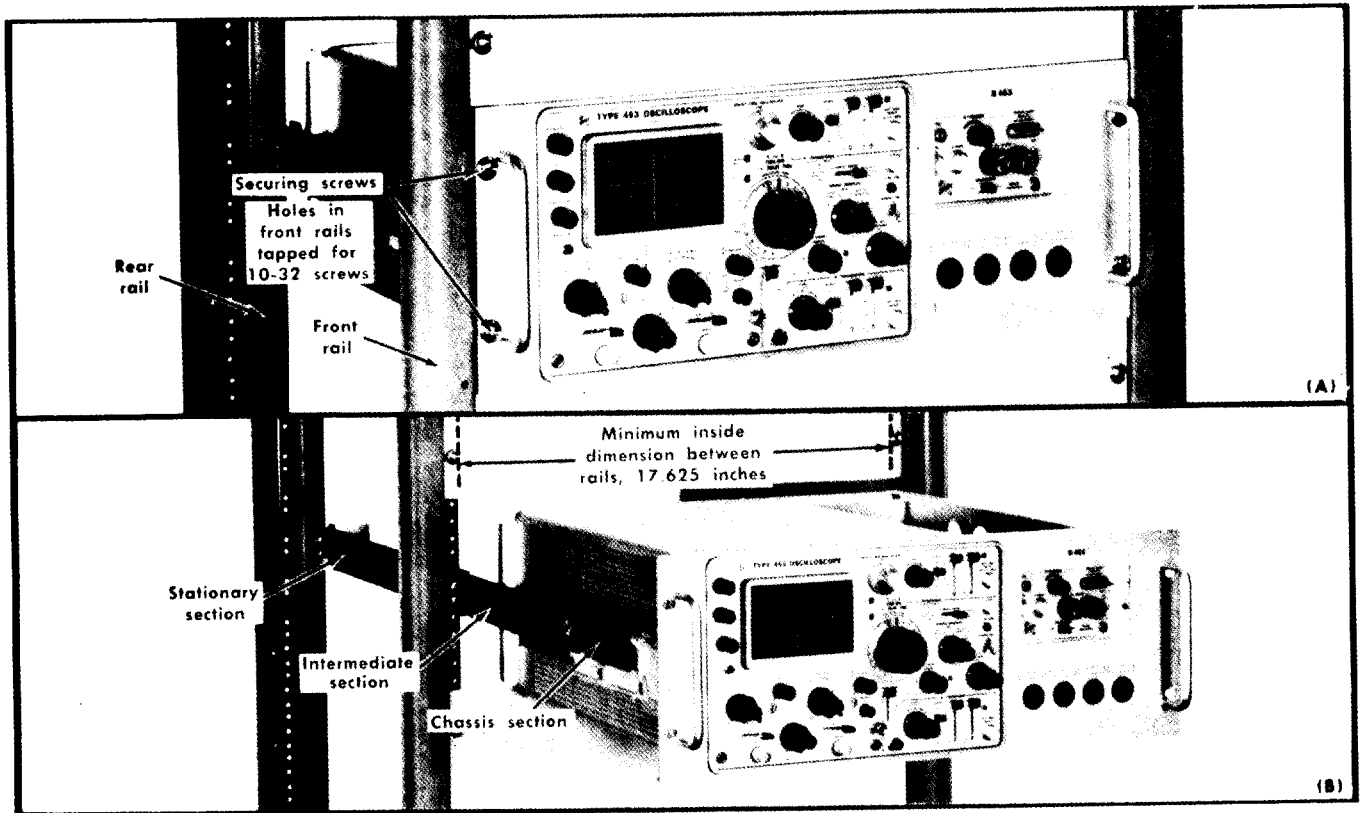
Fig. 10-1. The Type R453 installed in a cabinet rack (sides removed): (A) Held into rack with securing screws; (B) extended on slideout
