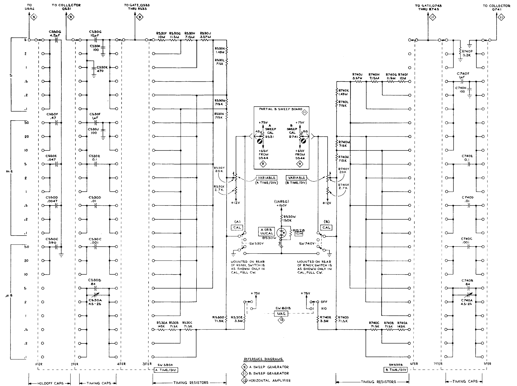
FIG. FO-22 A AND B TIMING SWITCH (S/N 20,000 & UP)
