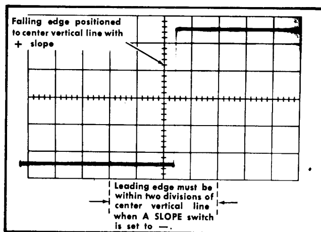
Fig. 5-29. Typical CRT display when checking calibrator duty cycle.
