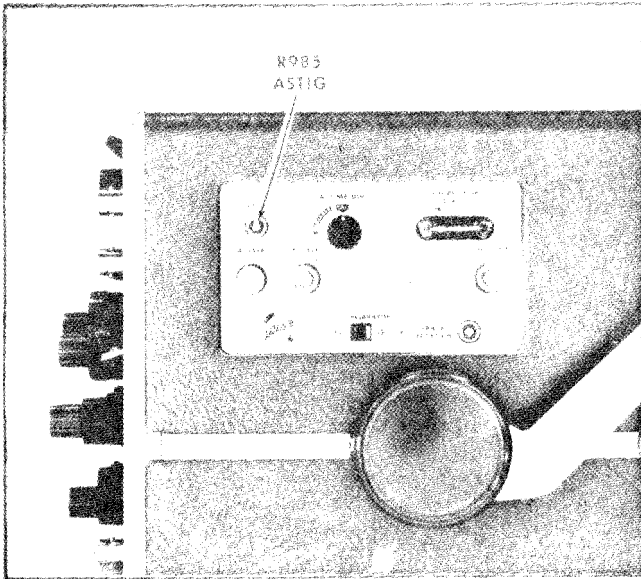
Fig. 6-11. Location of ASTIG adjustment (side panel)
