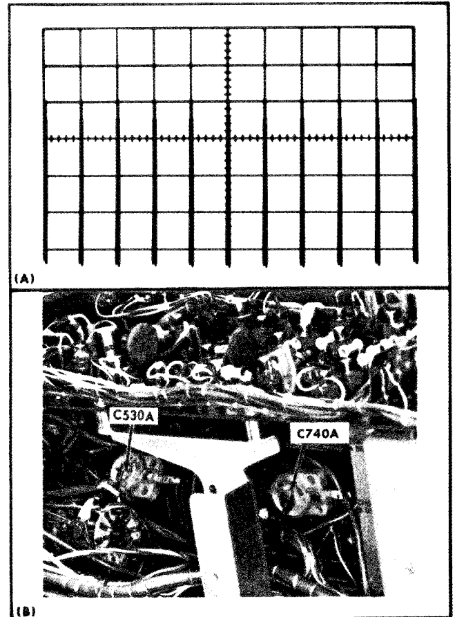
Fig. 6-45. Typical CRT display showing correct one-microsecond timing, (B) location of C530A and C740A (behind swing-out side panel).
