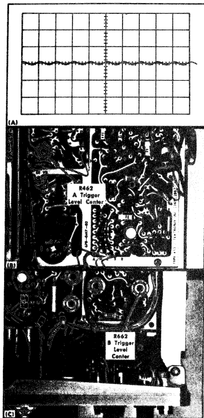
FIG. 6-29. (A) Typical CRT display when checking trigger level centering, (B) location of the A Trigger Level Center adjustment (A Sweep circuit board), (C) location of B Trigger Level Center adjustments of (B Sweep circuit board).
