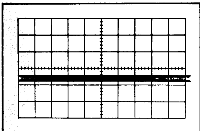
Fig. 5-8. Typical CRT display showing correct common-mode rejection ratio.
