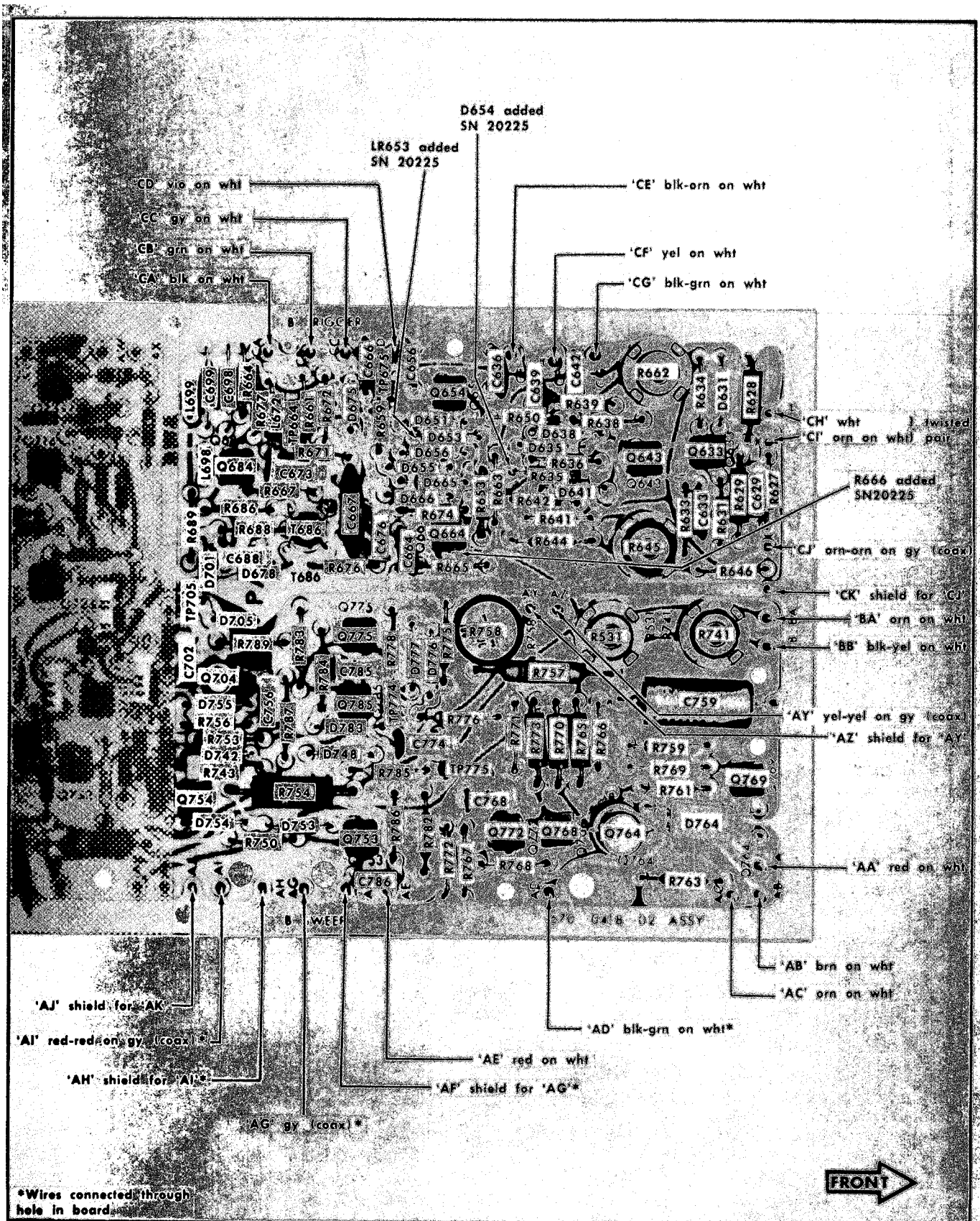
Fig. 4-14. Partial B Sweep circuit board. B Trigger Generator and B Sweep Generator circuits shown.
