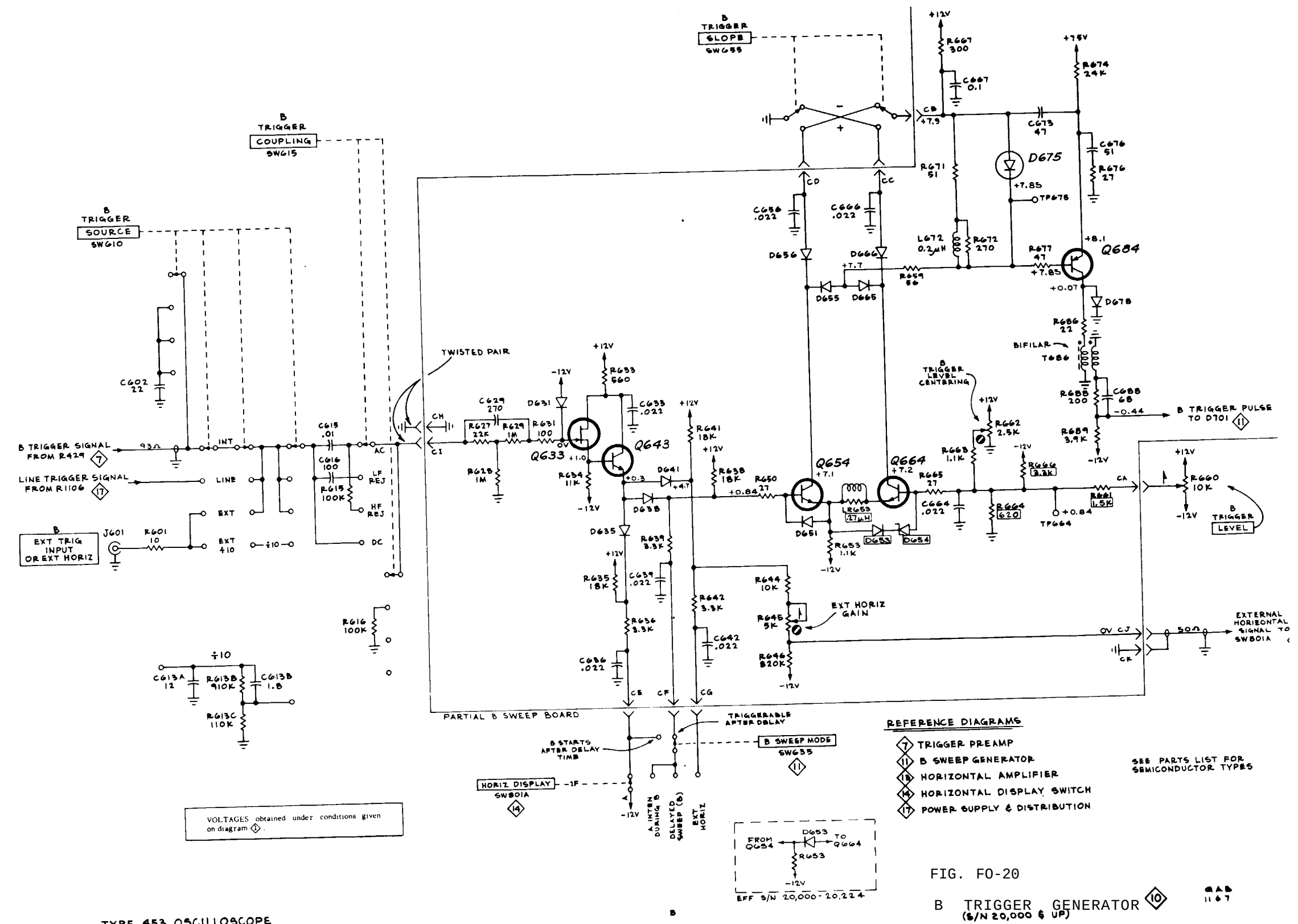
TYPE 453 OSCILLOSCOPE
